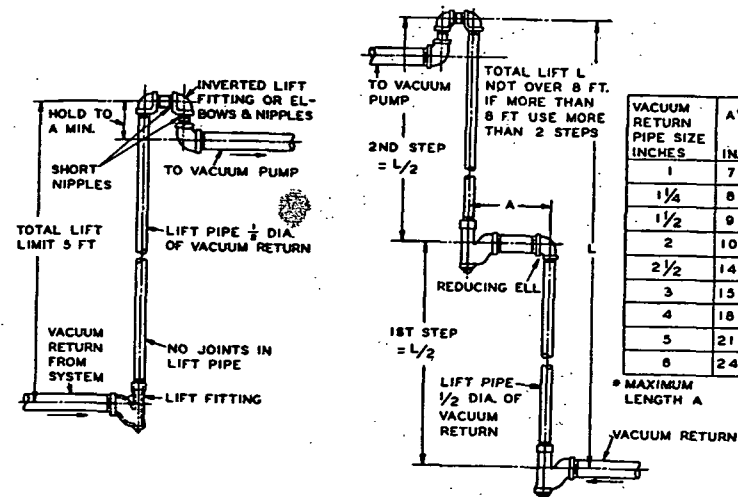
FIG. 17. METHOD OF CONSTRUCTING A LIFT IN A RETURN LINE
