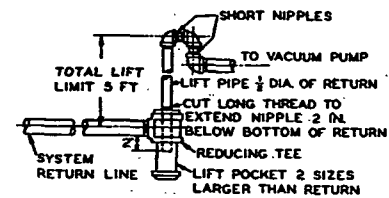
FIG. 19. HOW TO BUILD A LIFT FITTING
