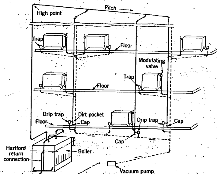
FIG. 16. TYPICAL DOWN-FEED VACUUM SYSTEM
