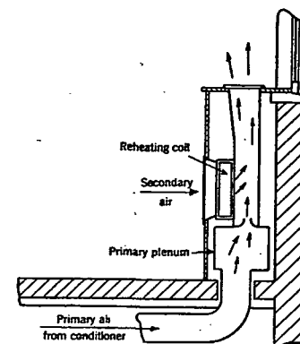
FIG. 4. INDUCTION UNIT (LOW PRESSURE TYPE)
