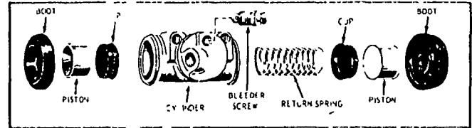
Figure 18—Typical Wheel Cylinder
