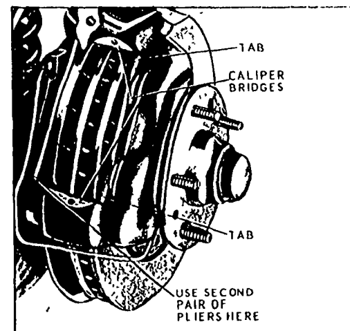
Figure 19—Removing Fixed Caliper Shoe and Lining
