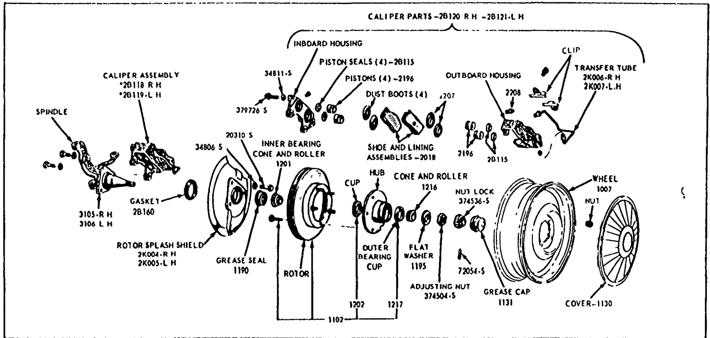
Figure 6—Fixed Caliper Disc Brake- Exploded View With Basic Part Numbers
