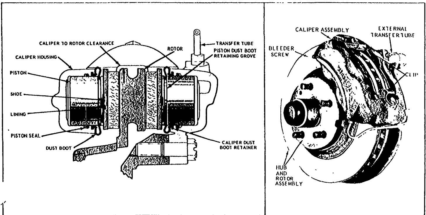
Figure 7—Fixed Caliper--Sectional View
