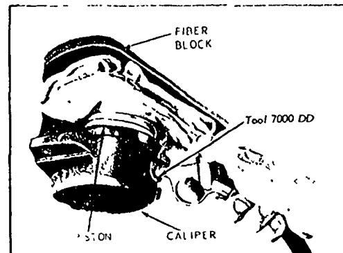
Figure 25- Using Air Pressure to Remove Piston
