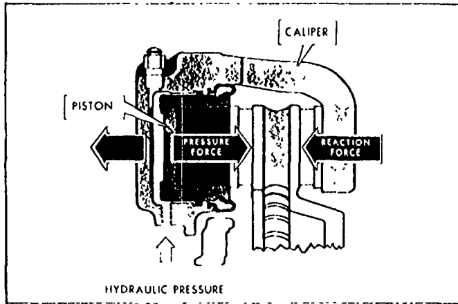
Figure 11—Floating Caliper Operation
