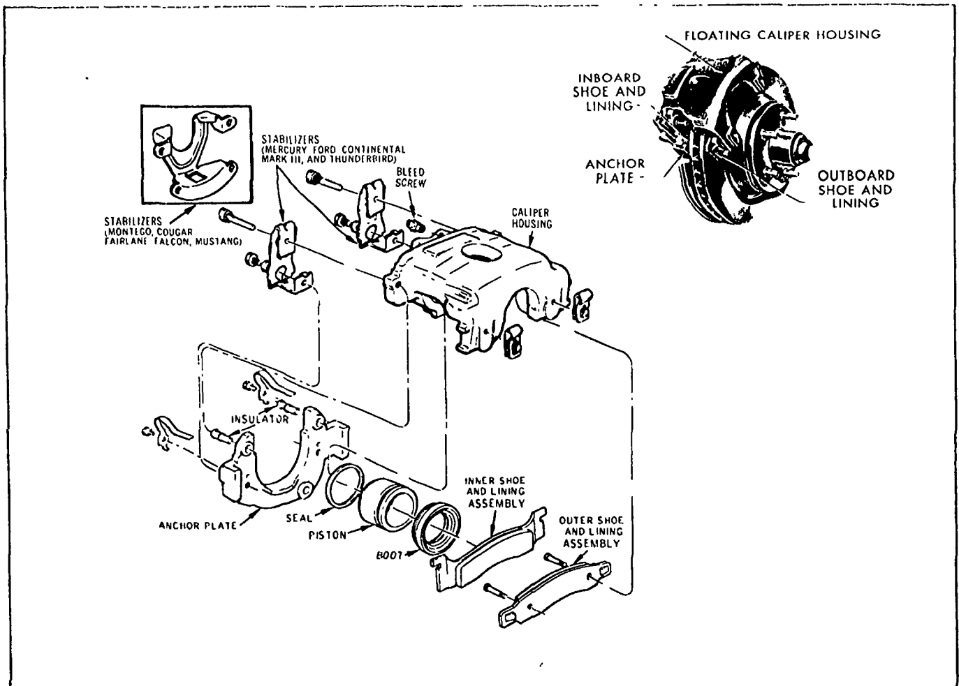
Figure 9- Floating Caliper Brake Assembly
