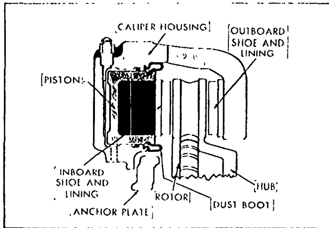
Figure 10—Floating Caliper Assembly—Sectional View
