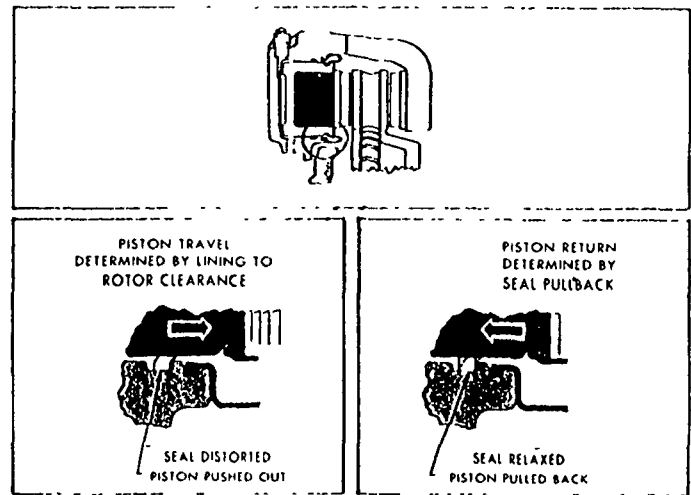
Figure 12—Caliper Piston Seals Control Self Adjustment
