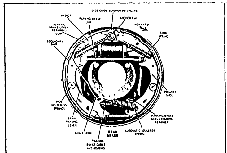
Figure 1--Duo Servo Brake Assemblies with Self Adjusting Mechanisms
