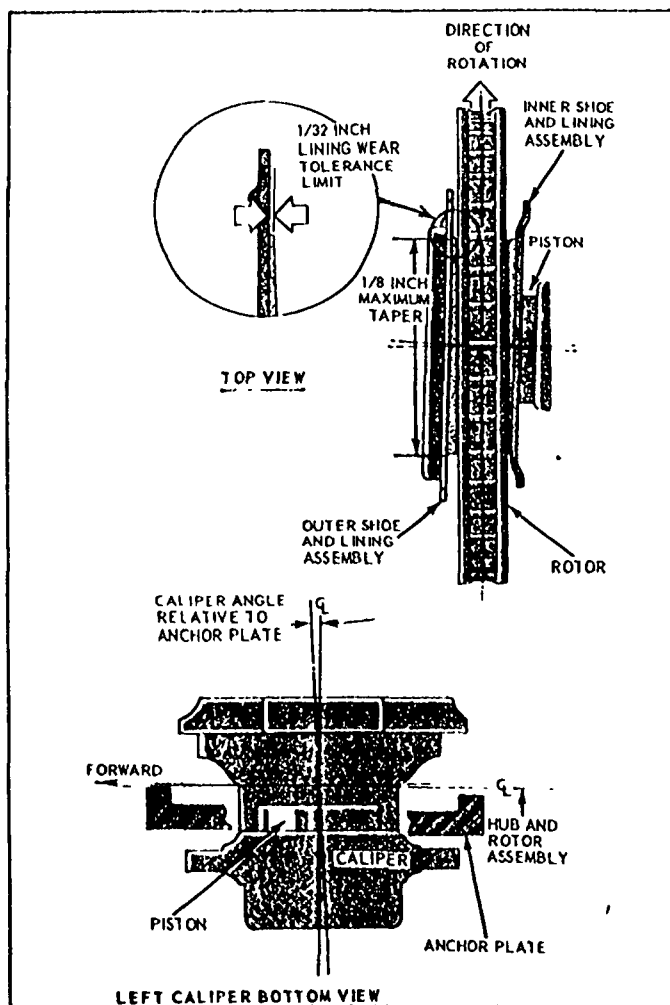
Figure 23- Taper Wear Pattern
