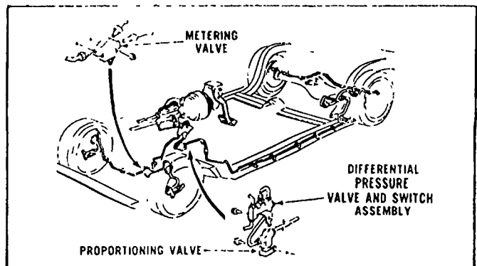
Figure 27— Dual Brake System
