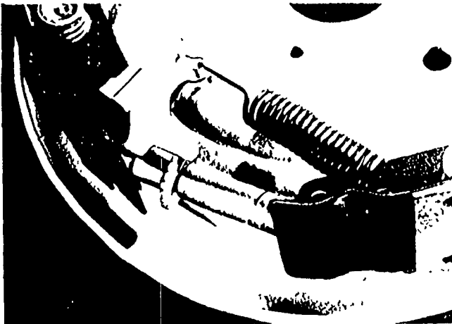
Figure 4- Adjusting Lever Moves Downward To Turn Star Wheel
