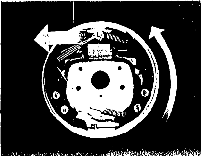
Figure 3--Secondary Shoe Movement Pulls Adjusting Lever Upward
