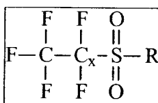
Figure 2. Schematic structure of PFAS.
