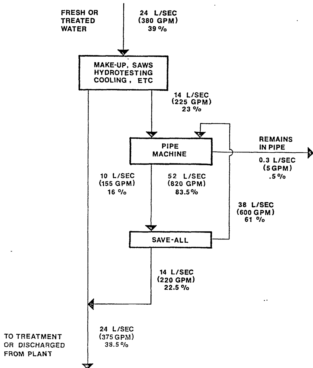
Figure 9 - Water Balance Diagram for a Typical Asbestos-Cement Pipe Plant
