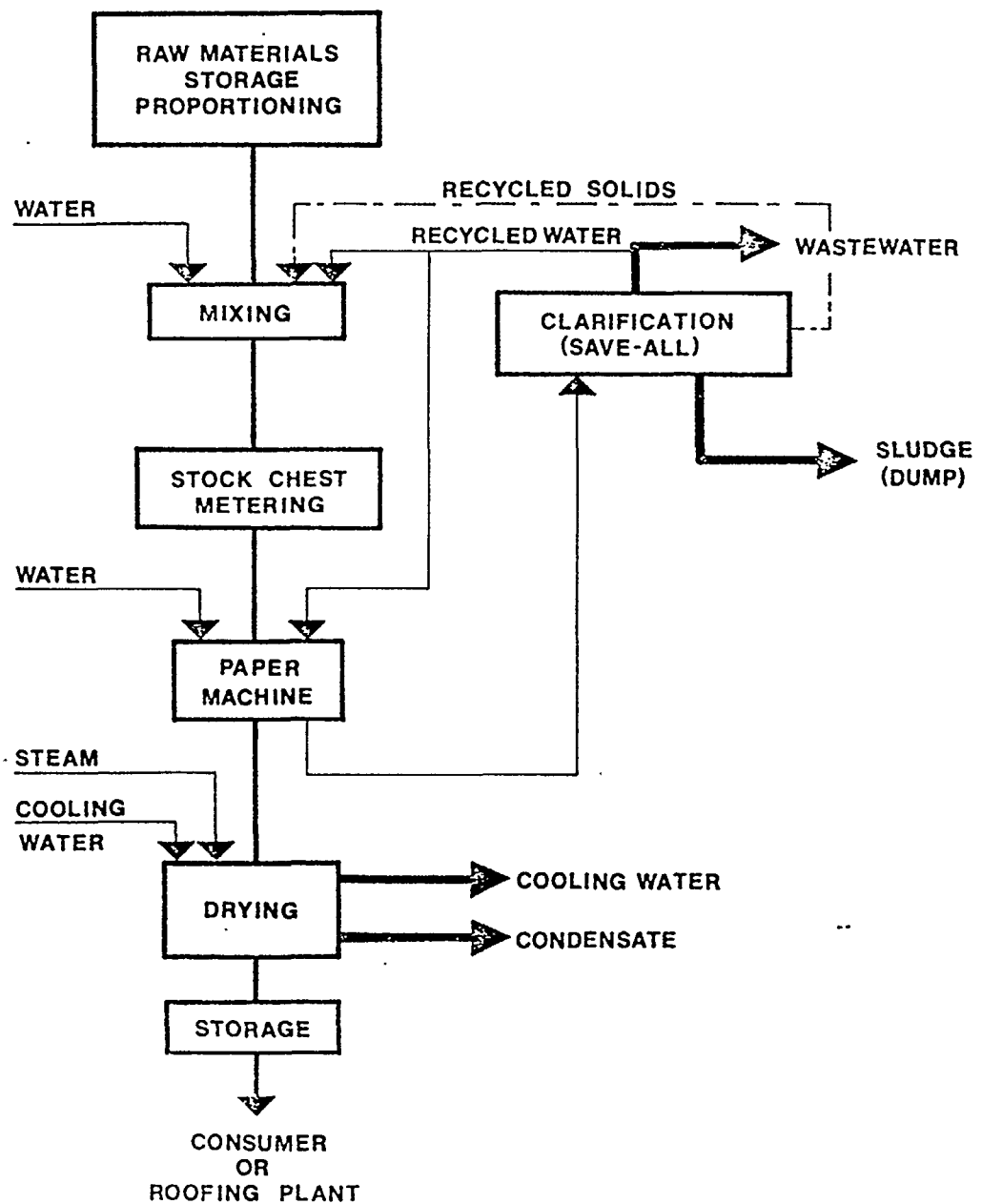
Figure 5 - Asbestos Paper Manufacturing Operations
