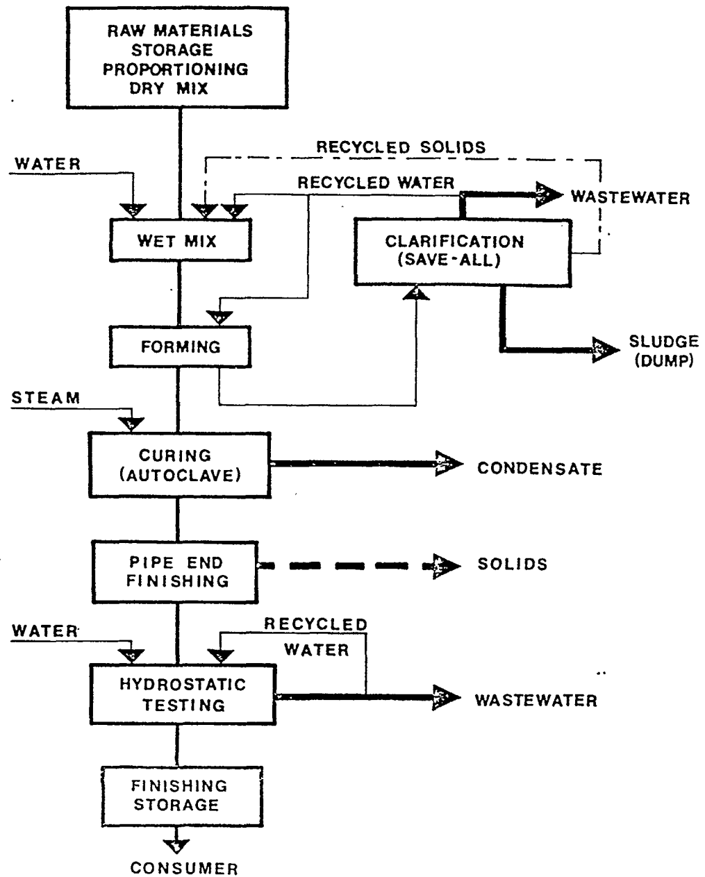
Figure 4 - Asbestos-Cement Pipe Manufacturing Operations, Wet Mechanical Process
