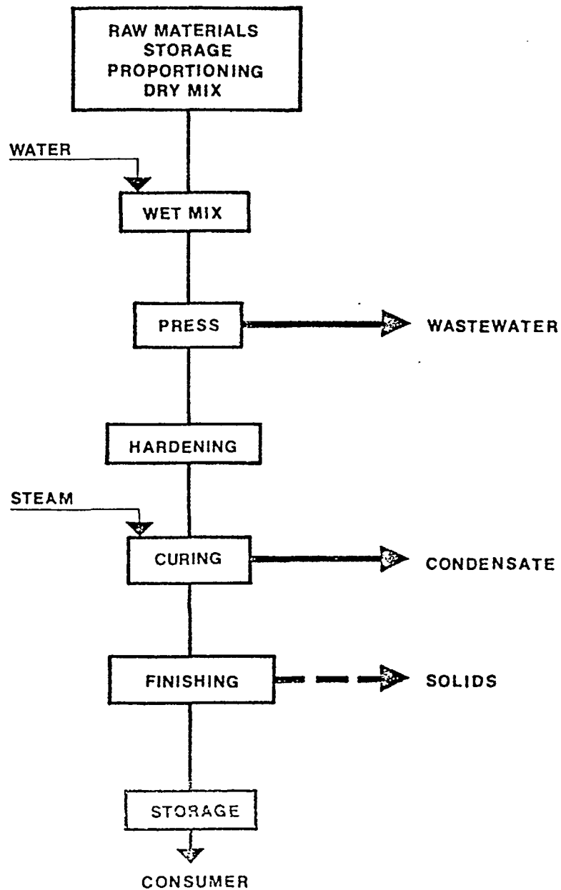
Figure 2 - Asbestos-Cement Sheet Manufacturing Operations, Wet Process
