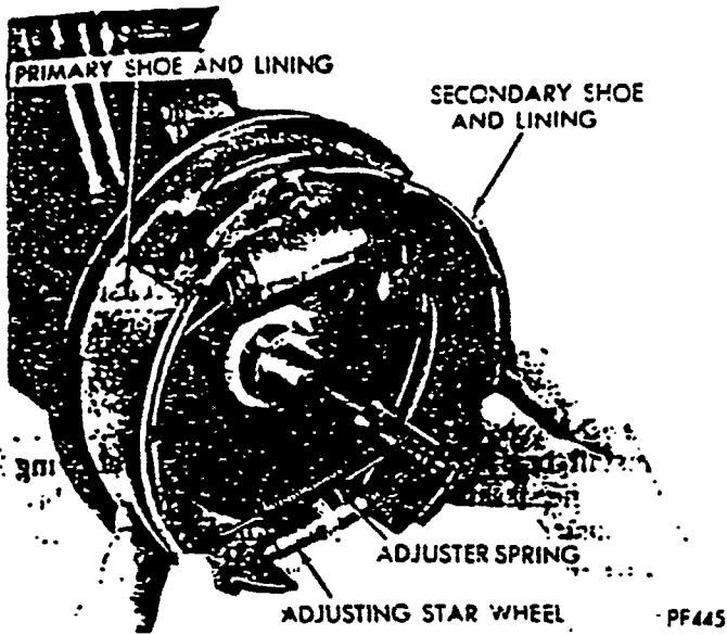
Fig. 12—Installing Brake Shoes—(Left Front)
