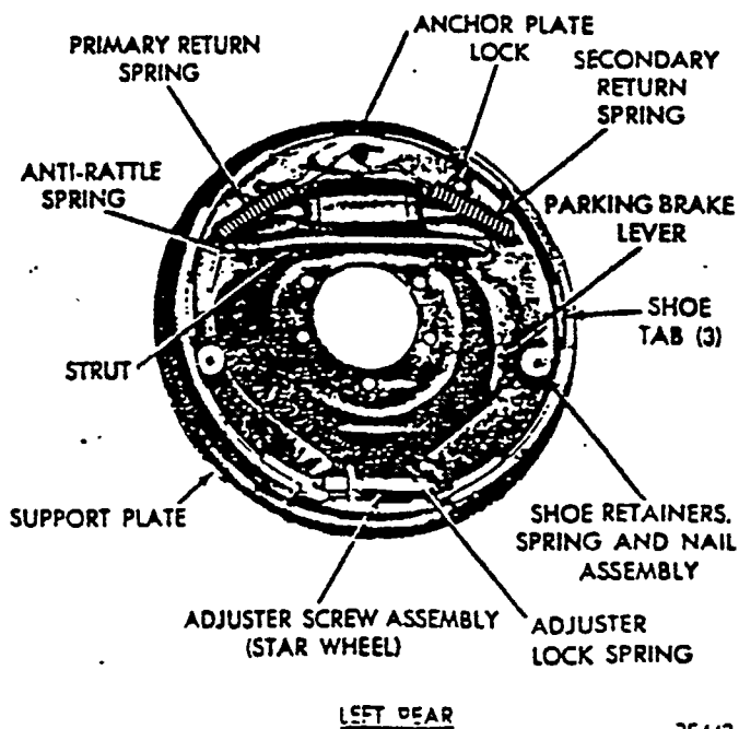
Fig. 6—Eleven Inch Brake Assembly—(Without Automatic Adjusters)—(Rear)
