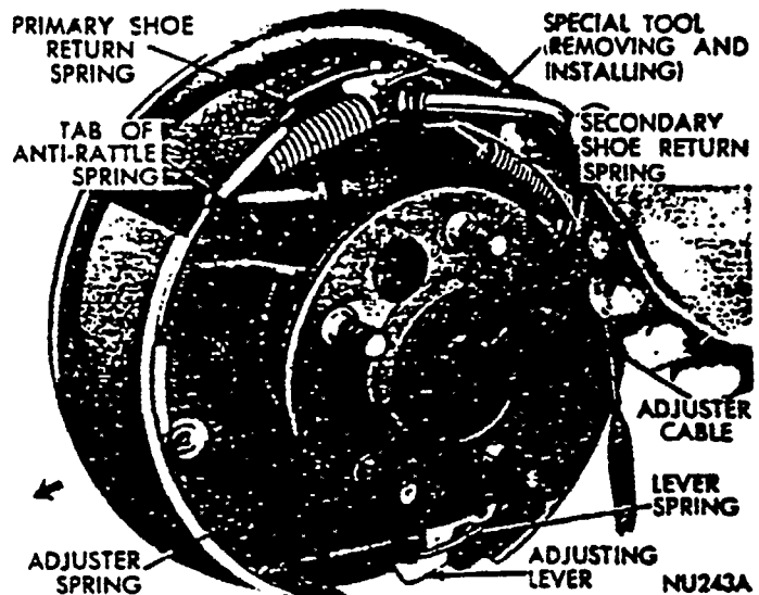
Fig. 7—Removing Shoe Return Springs—(Left Rear)
