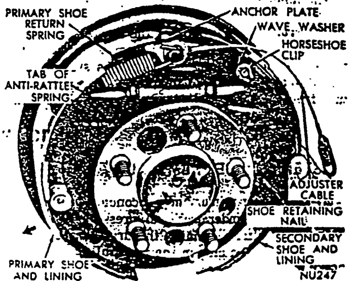
Fig. 14—Installing Brake Shoes—(Left Rear)
