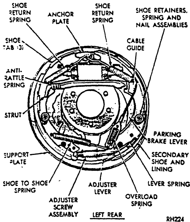
Fig. 2—Eleven Inch Brake Assembly
