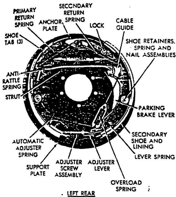
Fig. 5—Eleven Inch Brake Assembly—(Rear)
