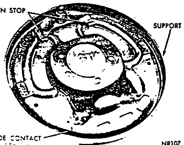
Fig. 11—Shoe Contact Area on Support
