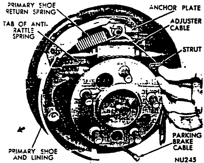
Fig. 13—Removing or Installing Parking Brake Strut and Spring—(Left Rear)
