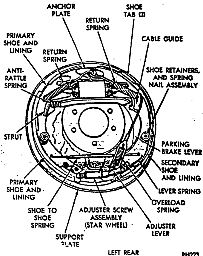
Fig. 1—Ten Inch Brake Assembly
