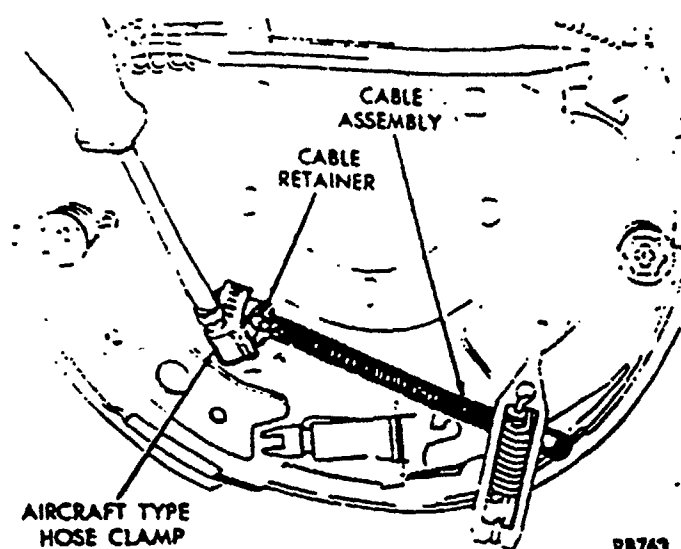
Fig. 10—Removing Brake Cable From Support Plate
