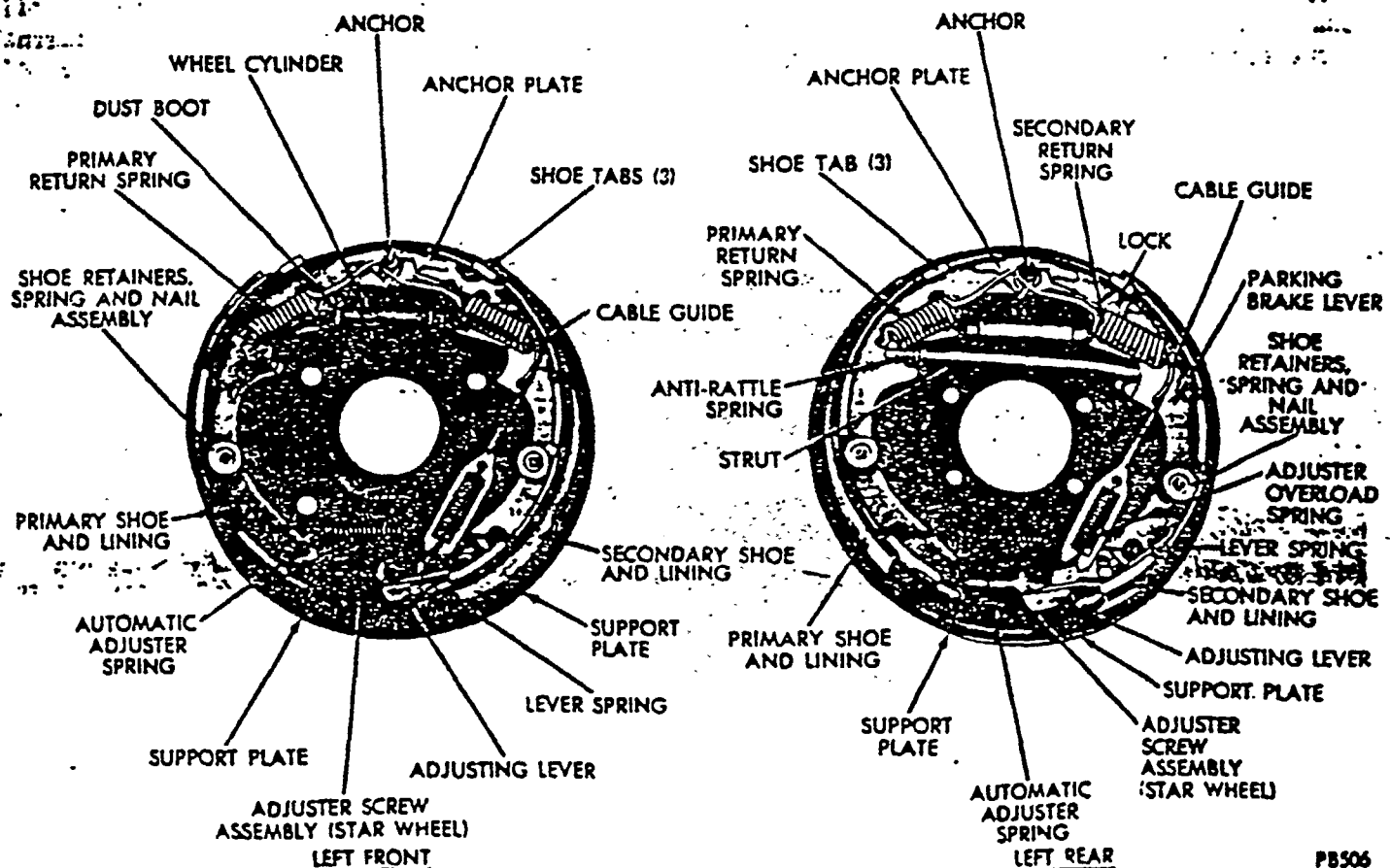
Fig. 1—Nine Inch Brake Assemblies
