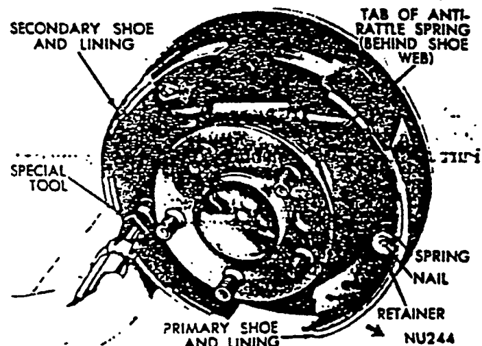
Fig. 8—Removing or Installing Shoe Retainers, Springs, or Nails—(Right Rear)
