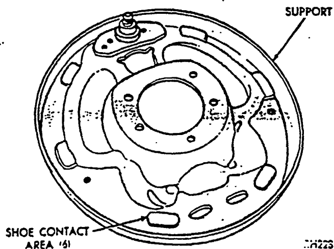
Fig. 7—Shoe Contact Pads on Support
