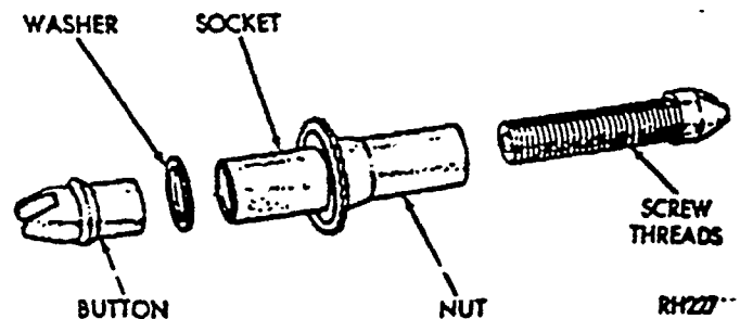
Fig. 5—Adjuster Screw Assembly
