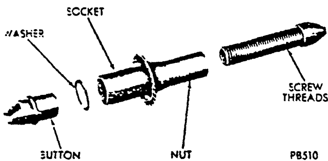
Fig. 9—Adjuster Screw Assembly
