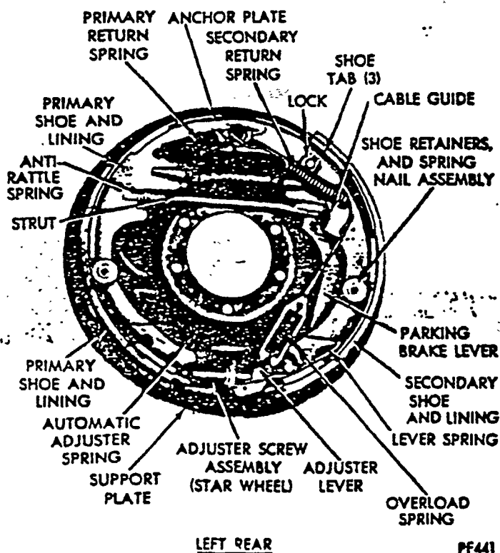
Fig. 4—Ten Inch Brake Assembly—(Rear)
