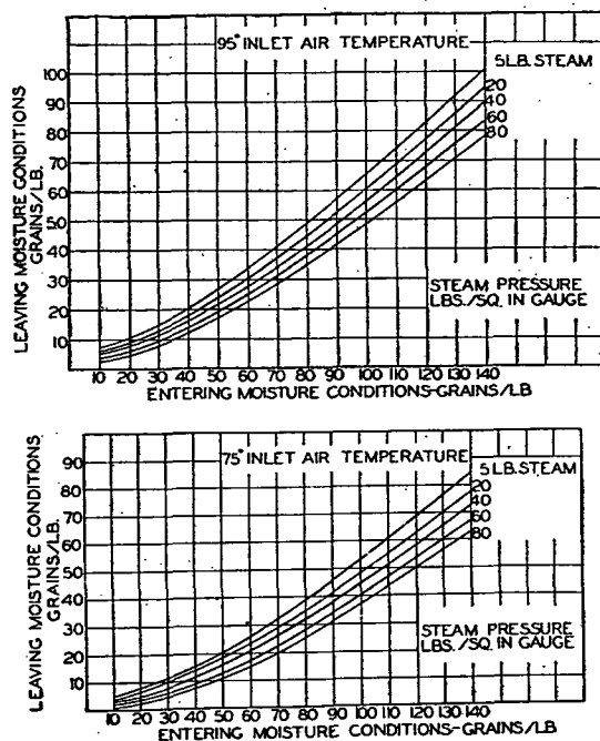
FIG. 8. SILICA GEL DEHUMIDIFIER PERFORMANCE DATA STEAM ACTIVATION TYPE
