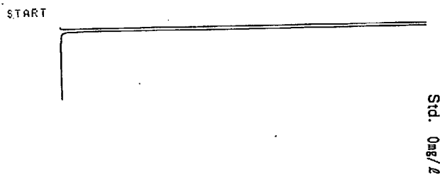
Figure 6.2 GC chromatograms of the test substance --- for calibration curve ---
