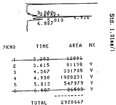
Figure 3.4 GC chromatograms of the test substance --- for measurement of concentration in water in Further investigation --- [1] after 2 days
