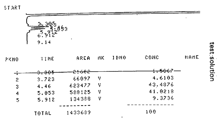
Figure 6.4 GC chromatograms of the test substance for measurement of mass of the trapped test substance
