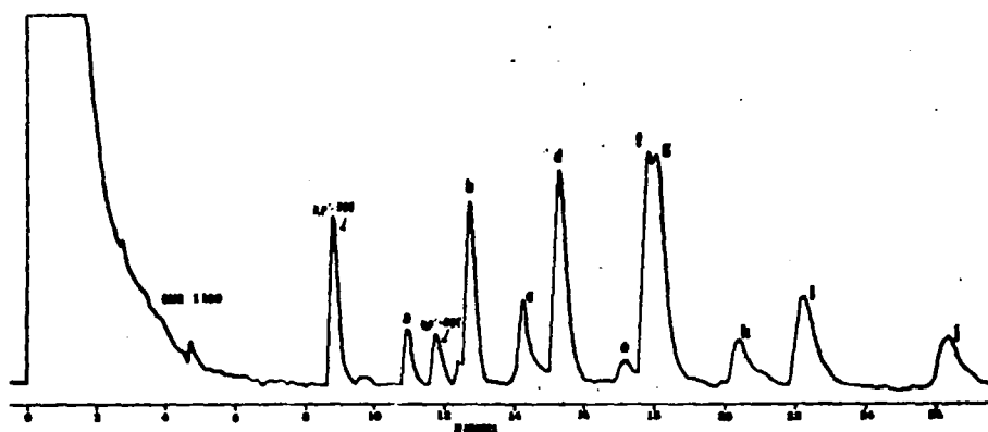
Figure 4. Total ion current monitor chromatogram of human adipose tissue extract B. Programmed temperature analysis: 2 min at 190°C, to 230°C at 5°C/min, isothermal at 230°C.
