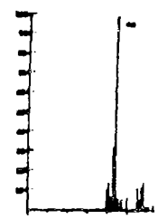
Figure 6. Aroclor 1260.
