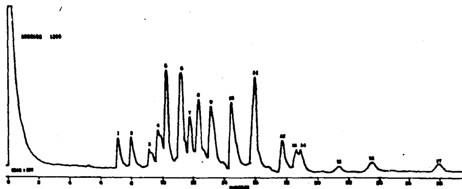
Figure 2. Total ion current monitor chromatogram of standard Aroclor 1260 mixture of polychlorinated biphenyls. Programmed temperature analysis: 2 min at 200°C, to 230°C at 5°C/min, isothermal at 230°C. (See text for remaining instrumental parameters and partial peak identification.)
