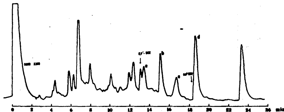
Figure 3. Total ion current monitor chromatogram of human adipose tissue extract A. Programmed temperature analysis: 5 min at 180°C, to 210°C at 5°C/min, isothermal at 210°C.
