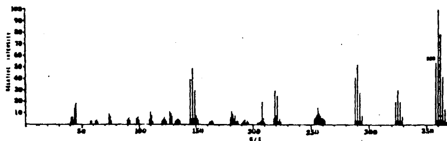
Figure 7. Mass spectrum of a hexachlorobiphenyl contained in human adipose tissue sample A (Peak d, Fig. 3).
