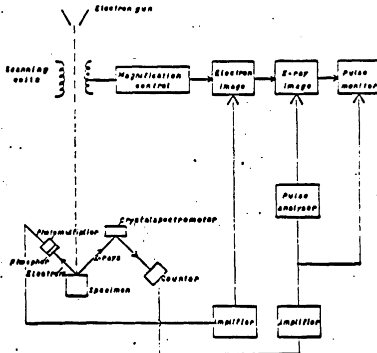
FIG. 1. Schematic diagram of microanalyzer. Example of an electron image Fig. 4a Example of a X-ray image Fig. 4b Example of the recording of the pulse monitor Figs. 5, 6, 7.
