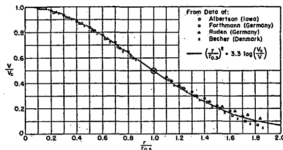
FIG. 4. CROSS-SECTIONAL VELOCITY PROFILES FOR STRAIGHTFLOW TURBULENT JETS
