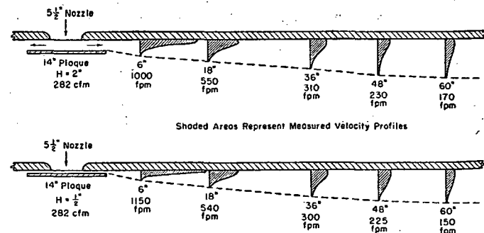
FIG. 5. AIR JETS FROM A 14-IN. CEILING PLAQUE FOR TWO SLOT WIDTHS WITH SAME RATE OF FLOW
