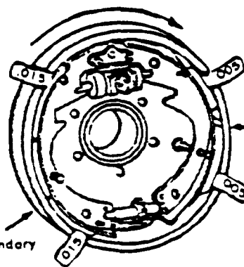
Bendix Dual-Servo
