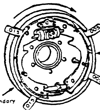
Bendix Dual-Servo
