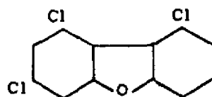
Trichlordiphenyl(ene) oxide or Trichlordibenzofurane
