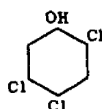
Trichlorophenol
