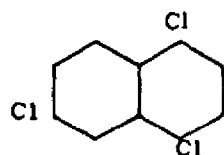
Trichloronaphthalene
