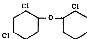
Trichlordiphenylether
