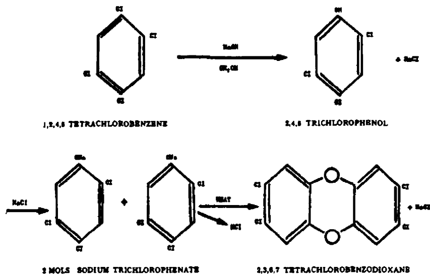
FIG. 3—Stages in formation of 2, 3, 6, 7-tetrachlordibenzodioxane
