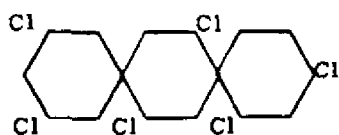
Hexachlorterphenyl
