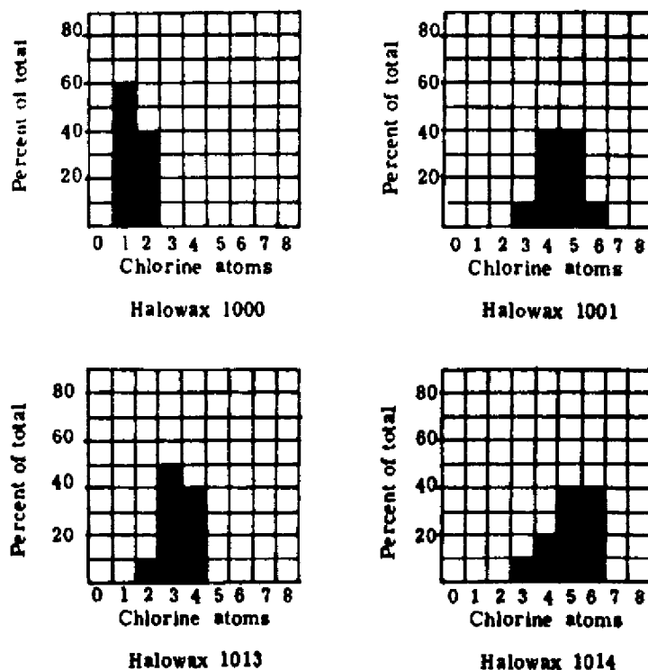
FIG 2 —Examples of four Halowax chlornaphthalenes
