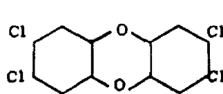
Tetrachlordibenzodioxane
