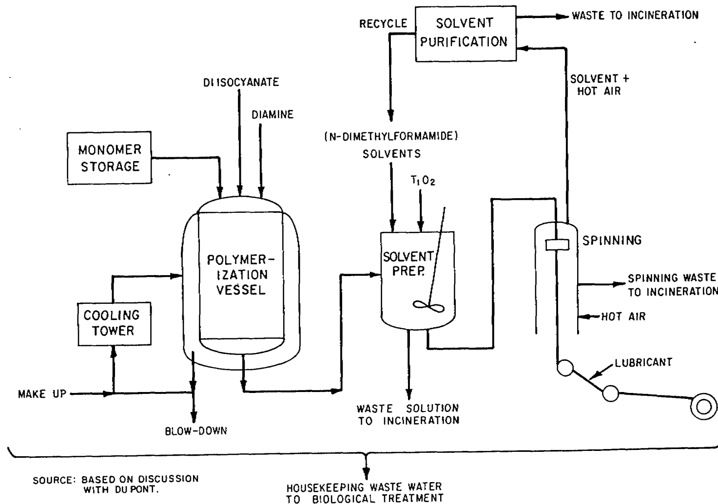
FIGURE III-51 SPANDEX FIBER PRODUCTION - DRY SPINNING PROCESS
