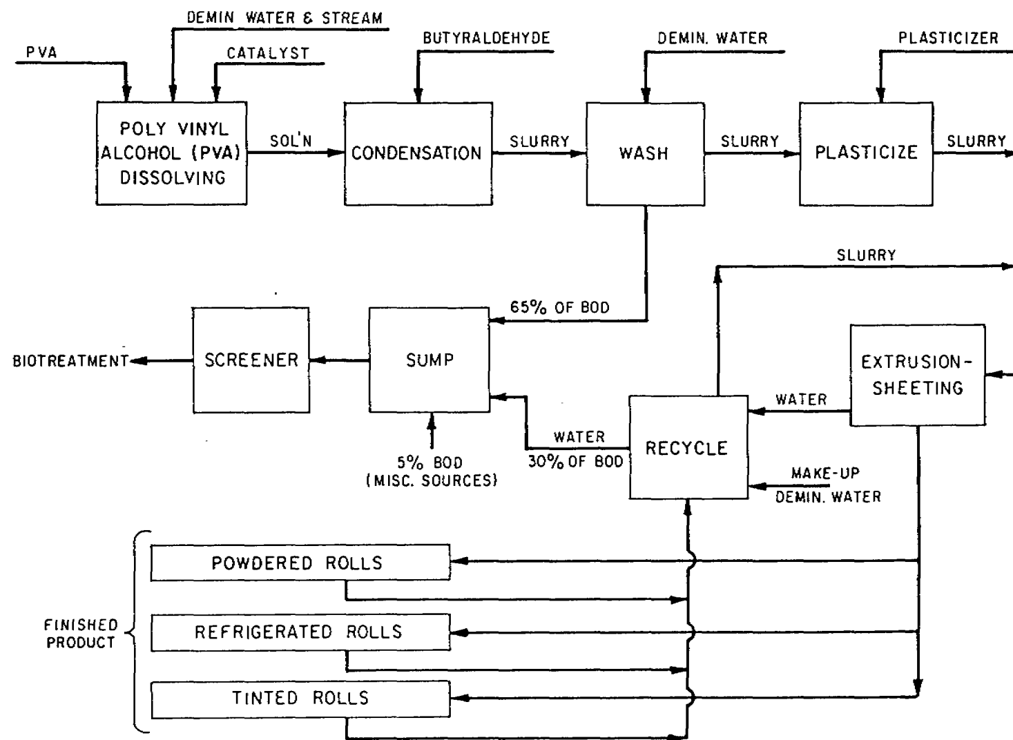
FIGURE III-39 POLYVINYL BUTYRAL PRODUCTION - DU PONT INC. PROCESS
