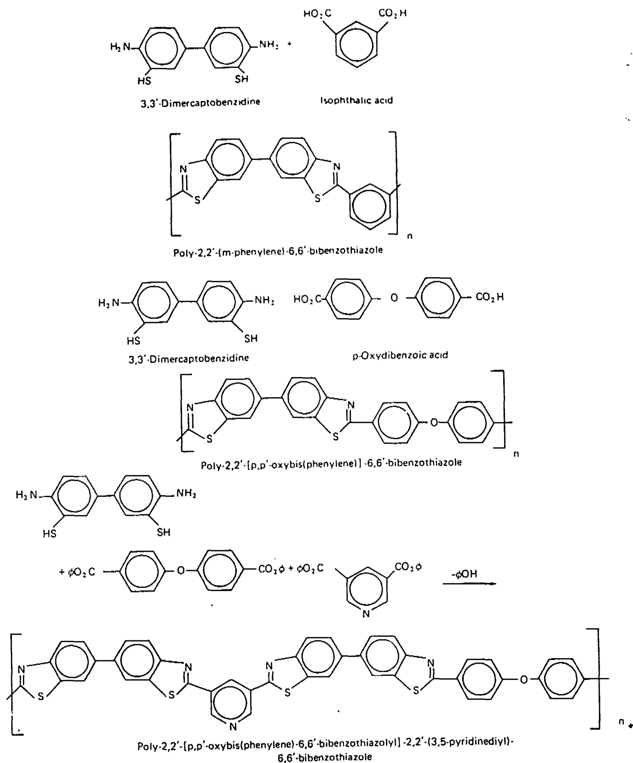
FIGURE III-23 TYPICAL STRUCTURES PRODUCED IN THE SYNTHESIS OF POLYBENZOTHAZOLES
