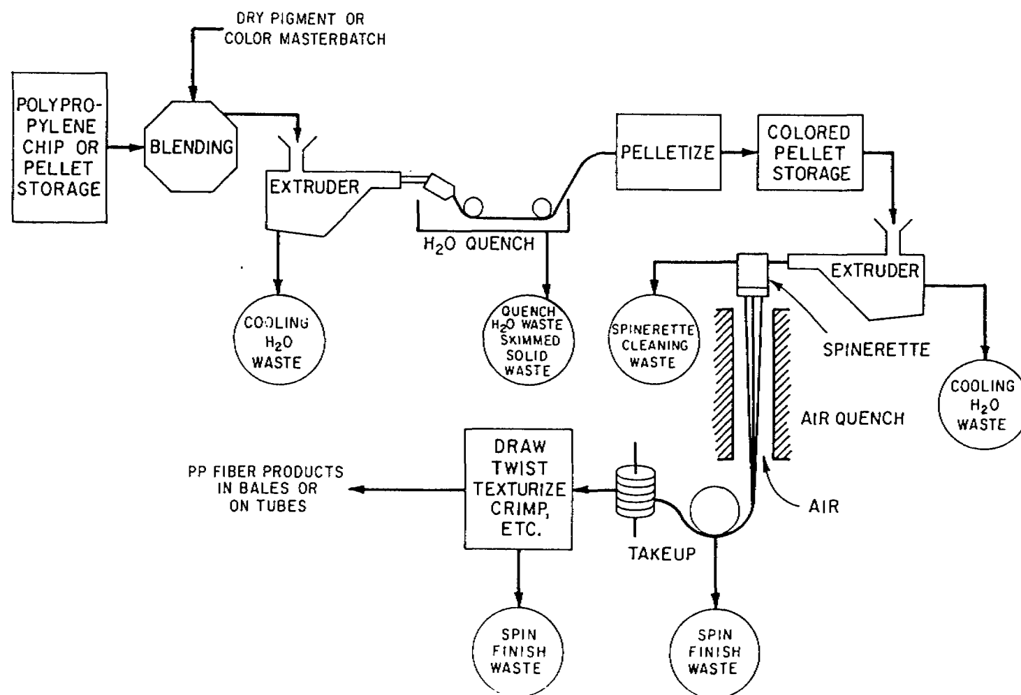
FIGURE III-34 POLYPROPYLENE FIBER PRODUCTION
