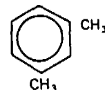
Meta-xylene
