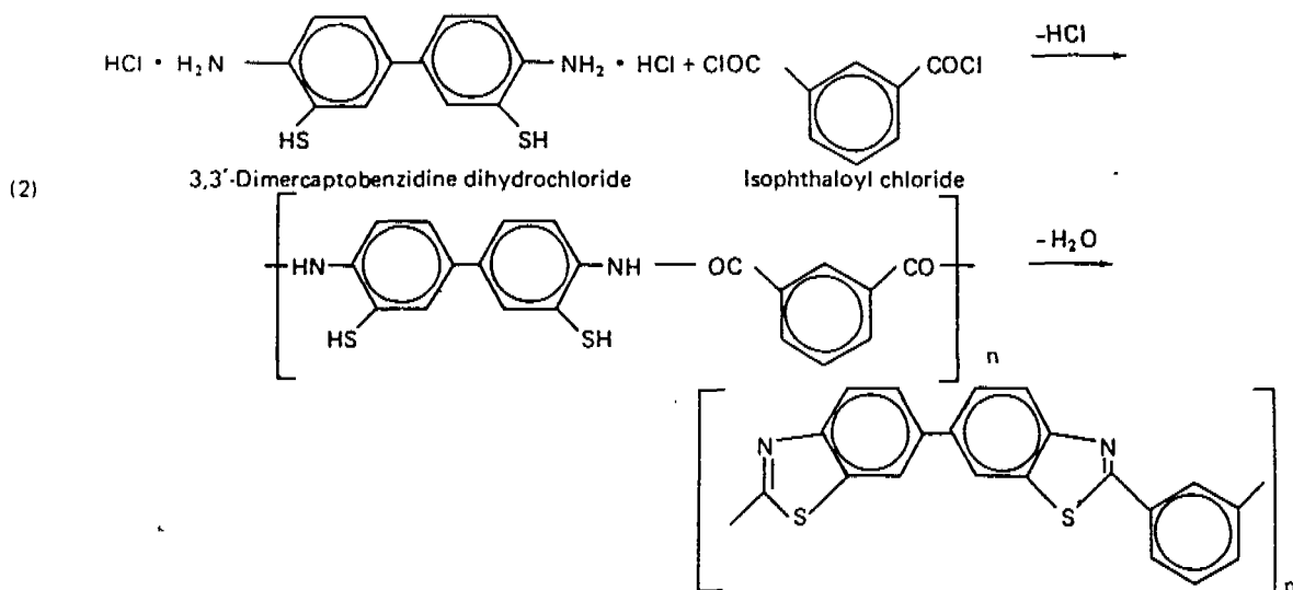
FIGURE III-22 TYPICAL REACTIONS TO FORM POLYBENZOTHAZOLES
