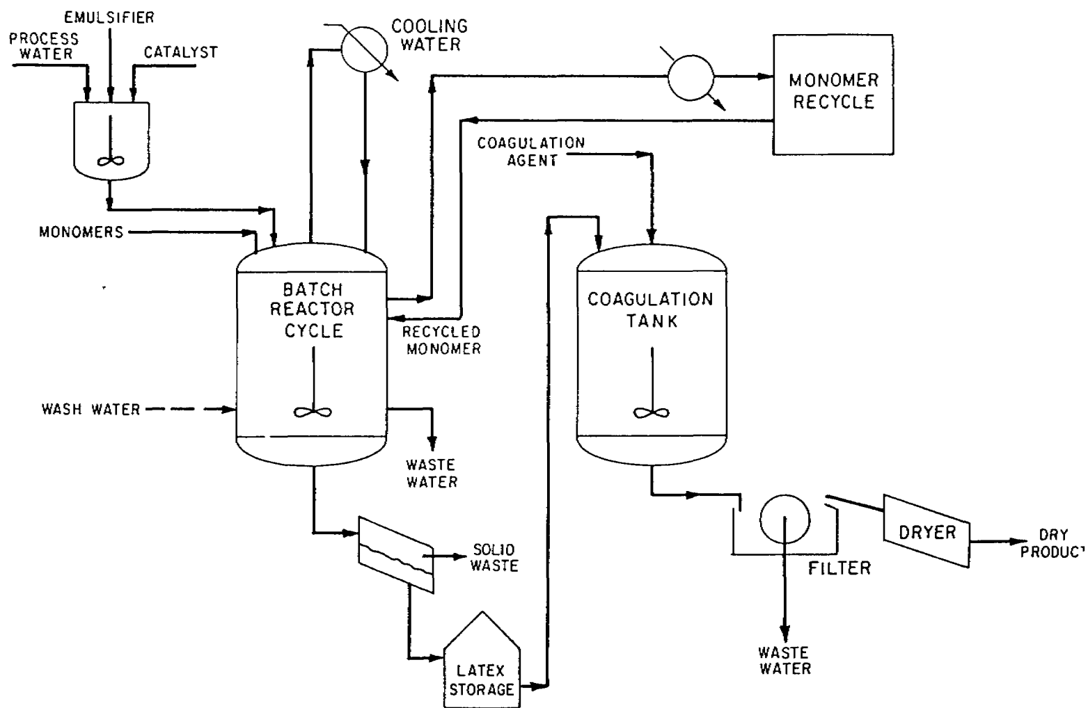
FIGURE III-16 NITRILE BARRIER RESIN PRODUCTION — EMULSION POLYMERIZATION PROCESS
