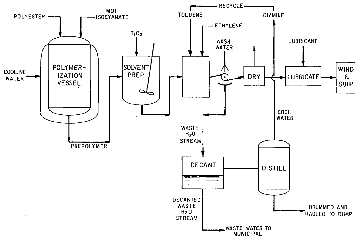
FIGURE III-53 SPANDEX FIBER PRODUCTION – REACTION SPINNING PROCESS
