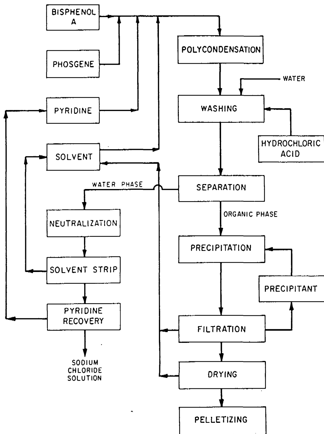
FIGURE III-27 POLYCARBONATE PRODUCTION – SEMI-CONTINUOUS PROCESS
