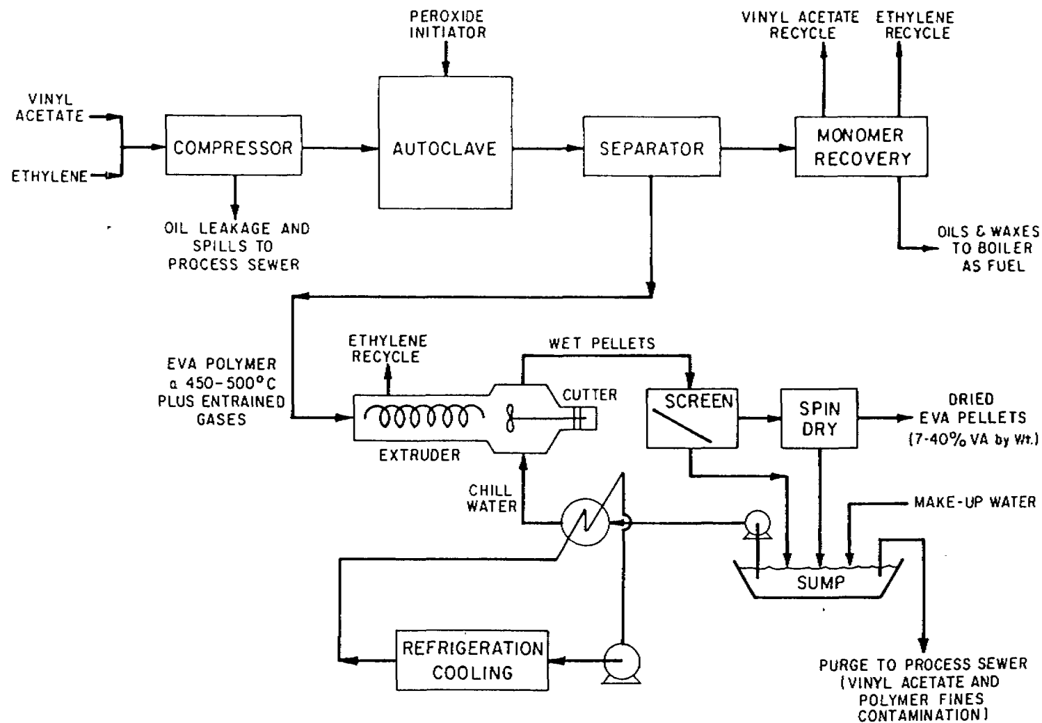
FIGURE III-12 ETHYLENE-VINYL ACETATE COPOLYMER PRODUCTION
