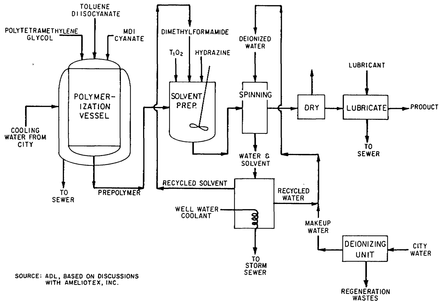
FIGURE III-52 SPANDEX FIBER PRODUCTION - WET SPINNING PROCESS
