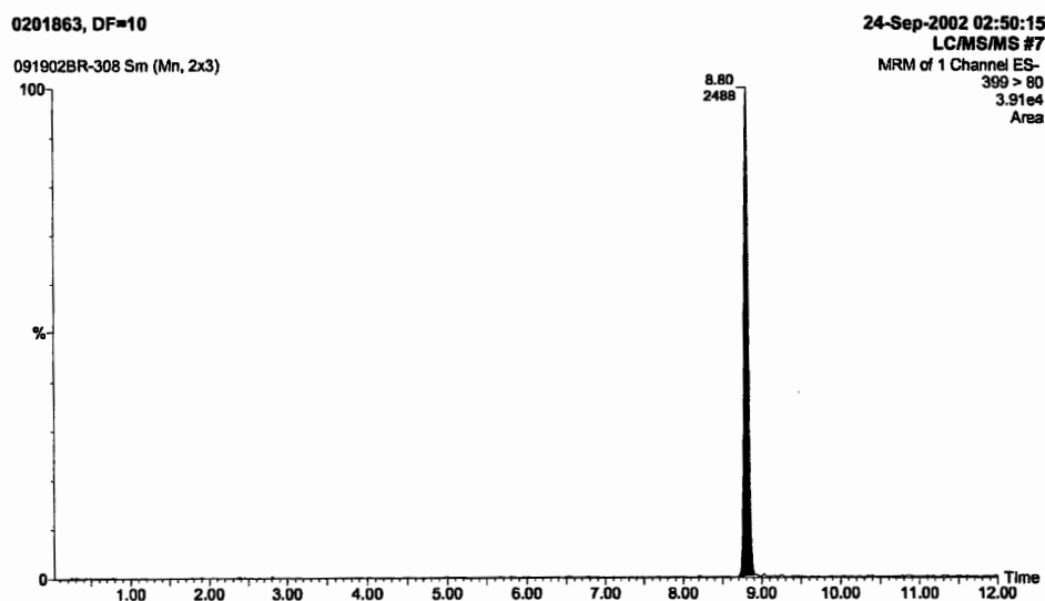
Figure 10. Chromatogram Representing Rat Serum Sample Analyzed for PFHS, DF=10 (Exygen ID: 0201863, Sponsor ID: 19079 GROUP II, Data Set: 091902BR)
