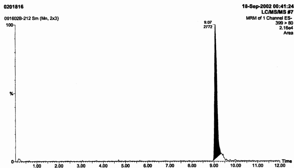
Figure 9. Chromatogram Representing Rat Plasma Sample Analyzed for PFHS (Exygen ID: 0201816, Sponsor ID: 19176 GROUP I, Data Set: 091602B)
