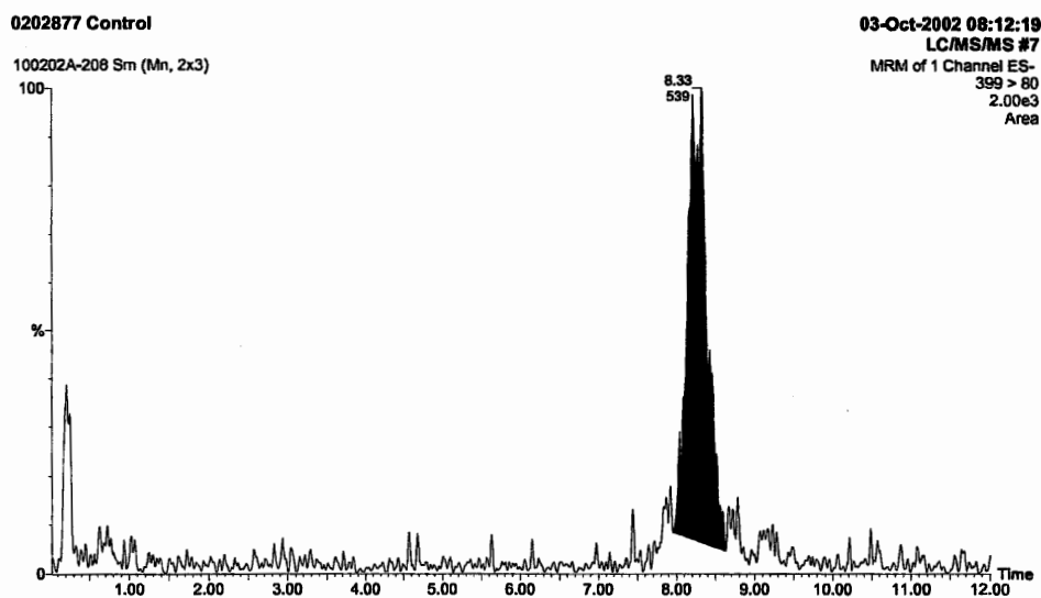
Figure 5. Chromatogram Representing a Control Rat Liver Sample for PFHS, (Exygen ID: 0202877 Control , Data Set: 100202A)
