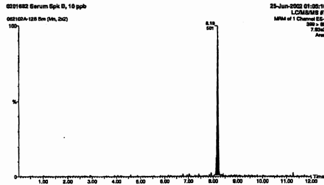
Figure 30. Representative Chromatogram of a Control Serum Sample Fortified at 10 ng/mL with PFHS
