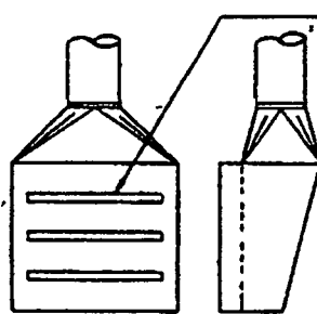
DISTRIBUTION BY SLOT (or baffles)
