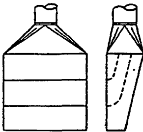
DISTRIBUTION BY SPLITTER VANES
