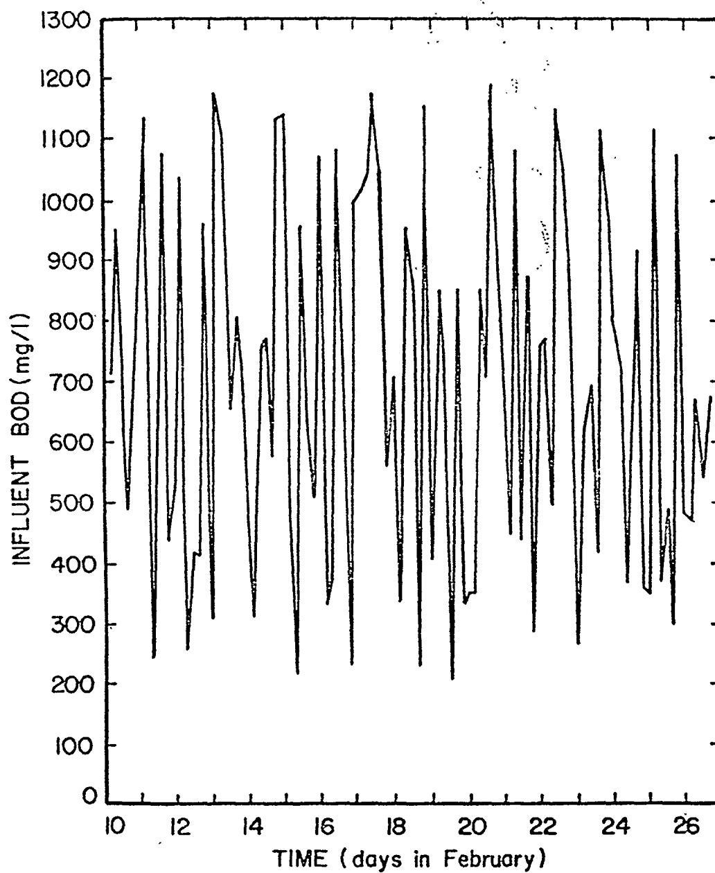
Figure 3-1. CHRONOLOGICAL VARIATION IN INFLUENT BOD CONCENTRATION
