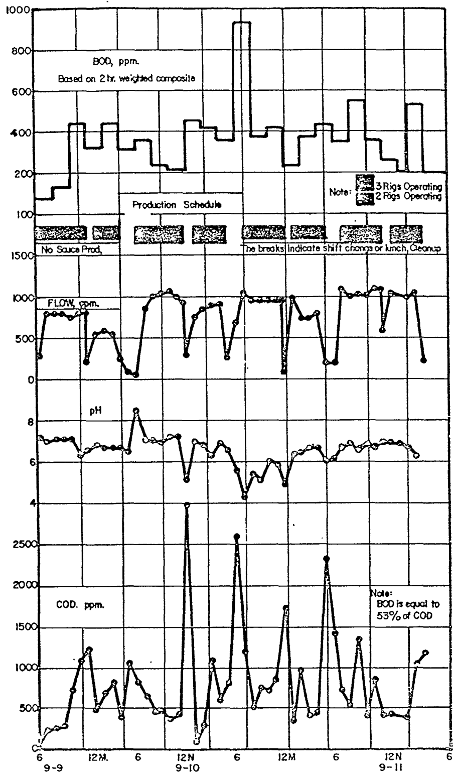
Figure 8-6. RAW DATA FROM WASTE SURVEY FOR TOMATO PROCESSING OPERATION
