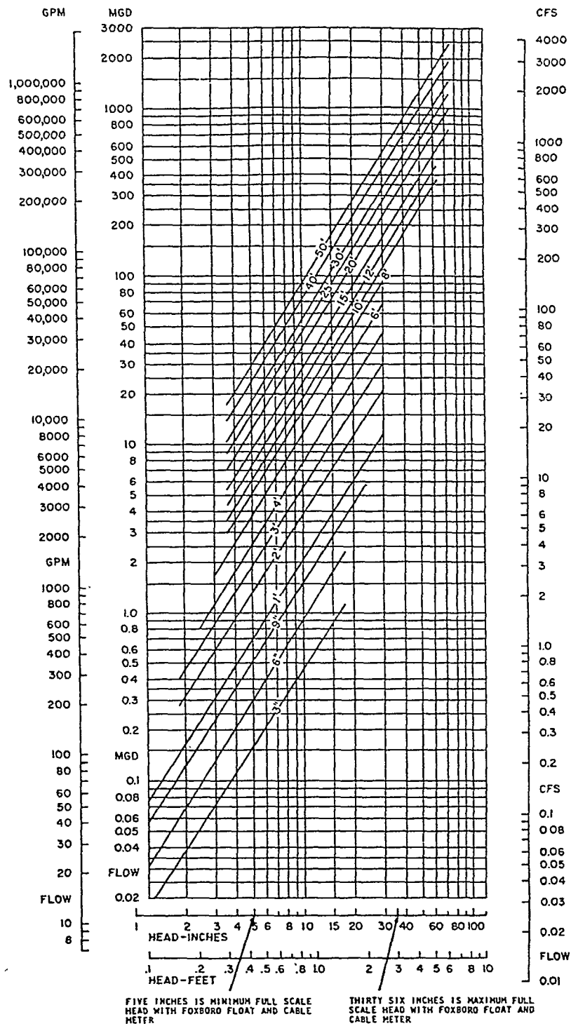
Figure 7-19. FLOW CURVES FOR PARSHALL FLUMES
