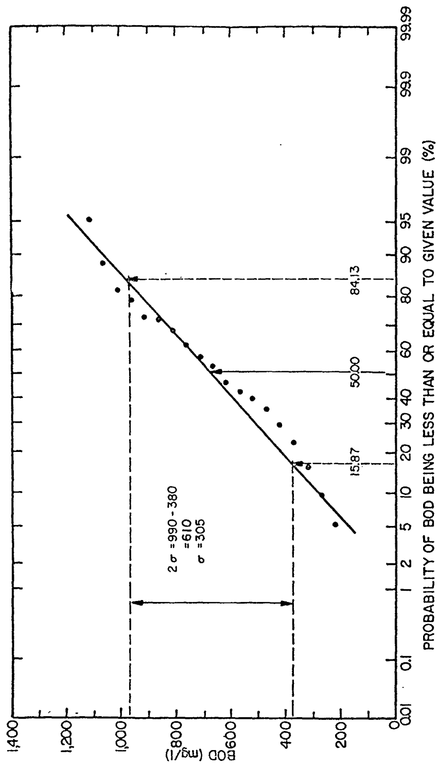
Figure 8-5. PROBABILITY PLOT OF GRAPHICAL METHOD II
