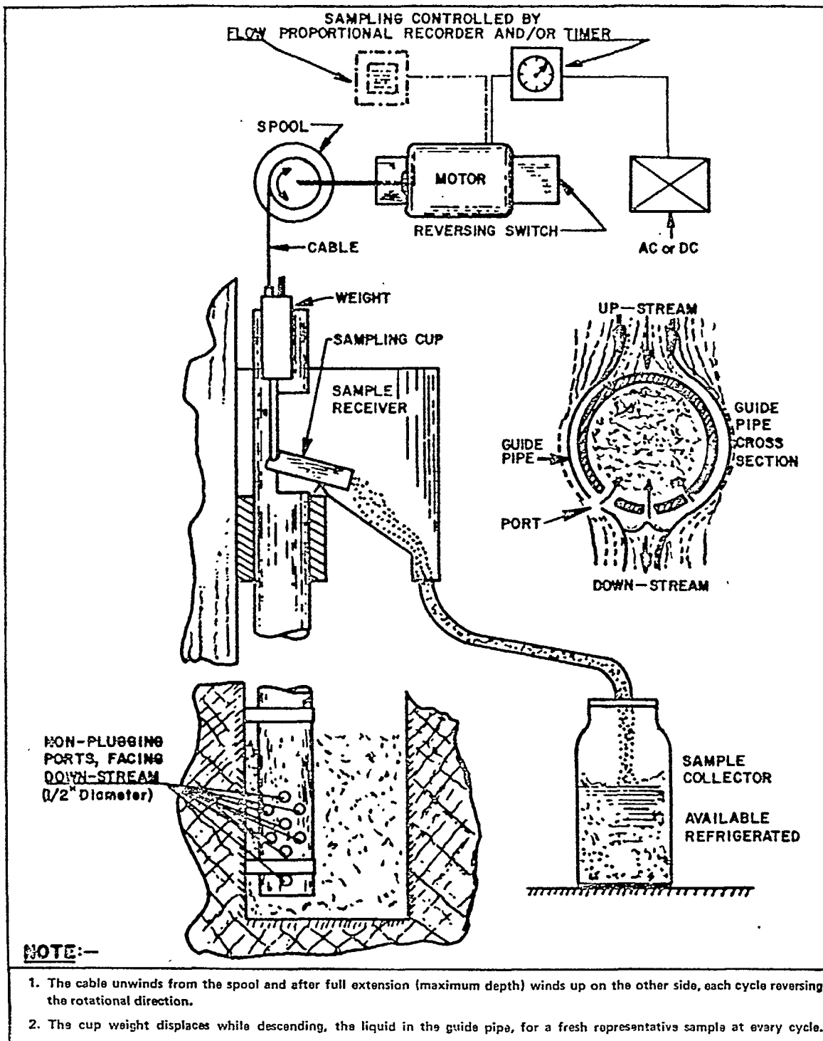
Figure 6-12. NON PLUGGING EFFLUENT VARY-SAMPLER (8)
