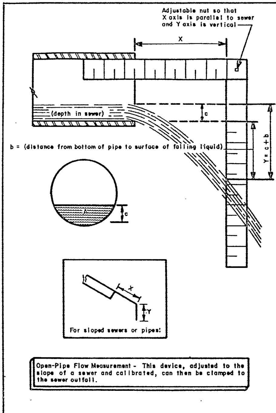
Figure 7-8. OPEN PIPE FLOW MEASUREMENT (4)
