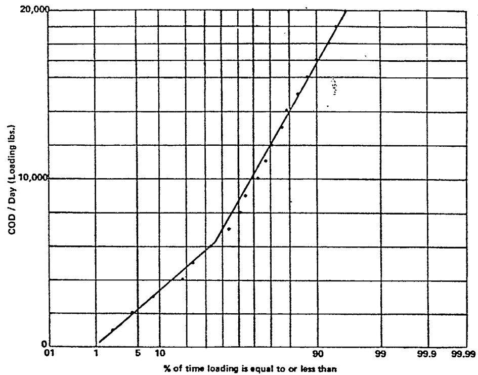
Figure 8-7c. PROBABILITY OF OCCURRENCE OF TOMATO WASTE LOADING
