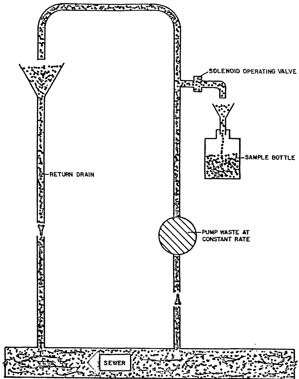
Figure 6-6. CONSTANT FLOW SYSTEM (6)
