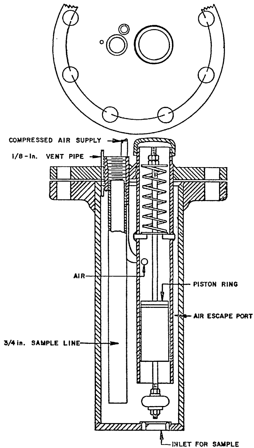
Figure 6-8. AIR LIFT AUTOMATIC SAMPLER (6)
