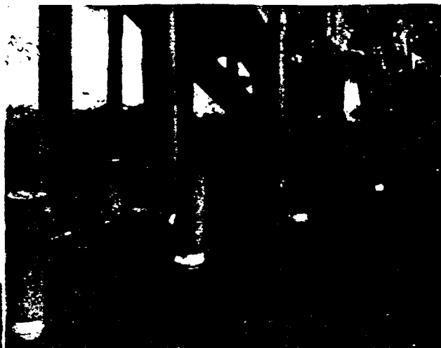
Lead bends and drum traps in a new toilet room in an office building in Tulsa, Oklahoma.
