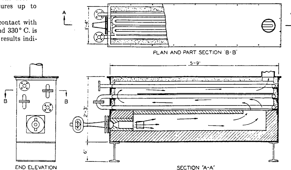
Figure 1. Heater
