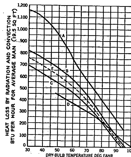
FIG. 6. RELATION BETWEEN RADIATION AND CONVECTION LOSS FROM THE HUMAN BODY AND DRY-BULB TEMPERATURE FOR STILL AIR a
