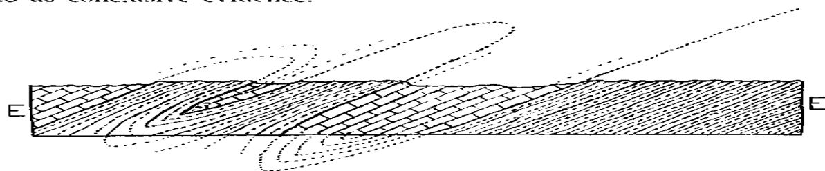
Figure 11 Section E—E, showing two infolded minor synclines of limestone, between anticlines of garnet-gneiss, on the flank of the great fold of garnet-gneiss which is partially represented at the right.
