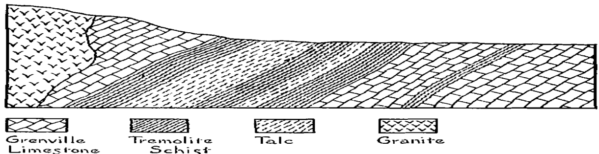
Figure 16 Generalized section of the Edwards talc deposits
