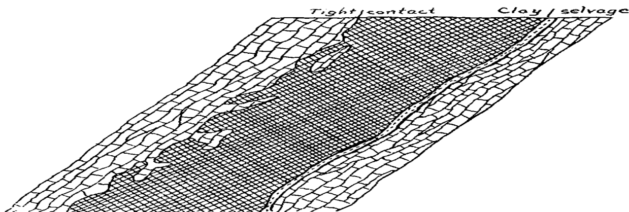
Figure 15 Relation of ore and limestone in No. 1 mine, Northern Ore Company.
