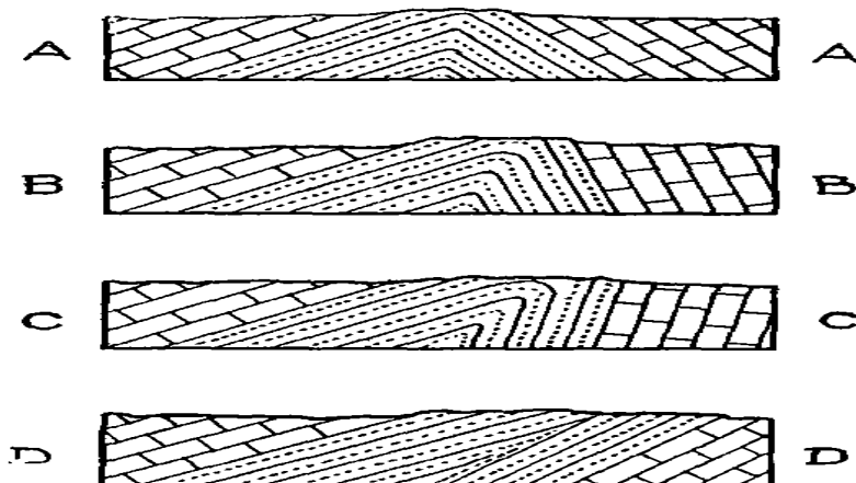
Figure 10 Sections A, B, C, and D across the end of the pitching fold of garnet-gneiss.
