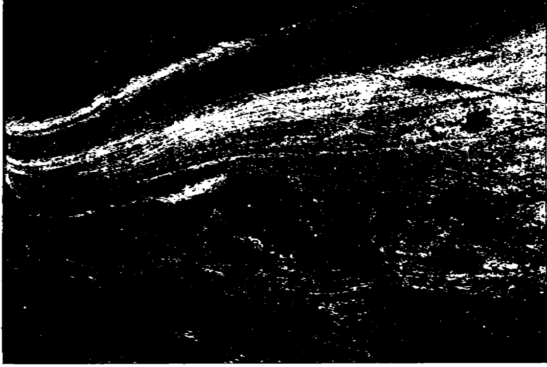
Folding and banding of impure Grenville limestone, Edwards.
