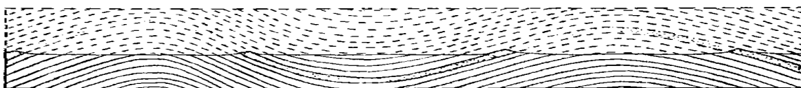
Figure 5 Diagram of gently folded beds which have been truncated by erosion, the upper dotted portion having been worn away; showing the broadly open character of the folds and the dips in opposite directions of the two limbs.
