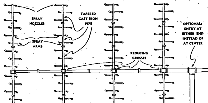
FIG. 4. TYPICAL NOZZLE ARRANGEMENT FOR A SPRAY POND
