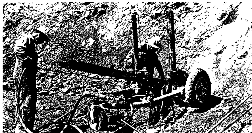
Churn drill rig and crew preparing for a "shot"
