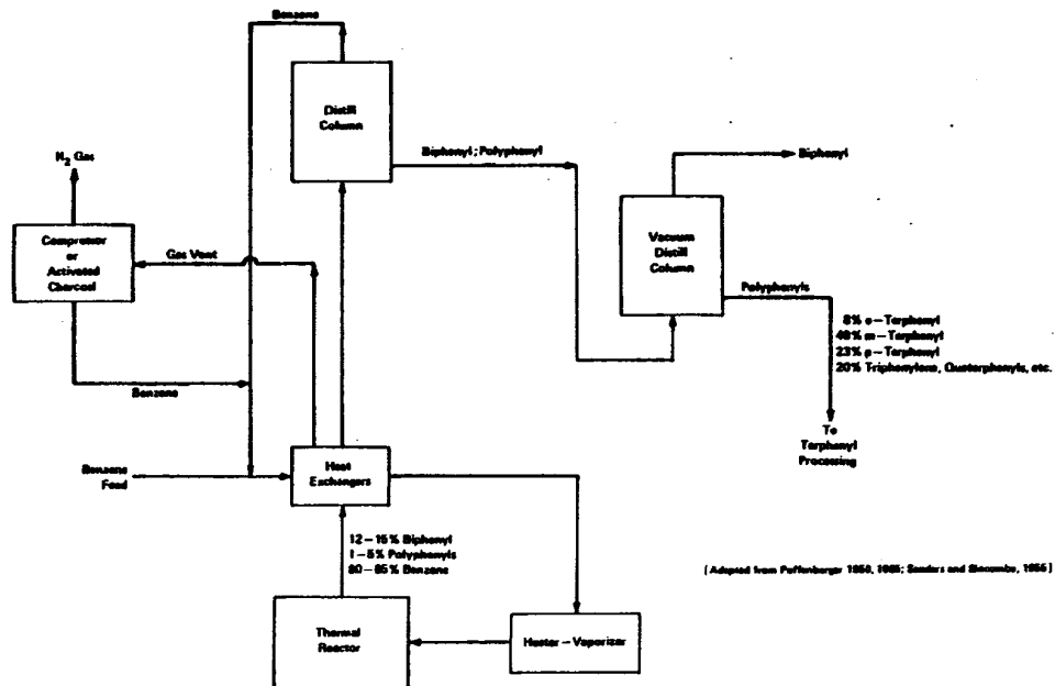
Figure IV-1. Biphenyl From Thermal Dehydrogenation of Benzene
