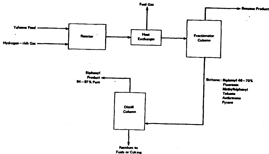
Figure IV-2. General Process for Hydrodealkylating Toluene to Benzene
