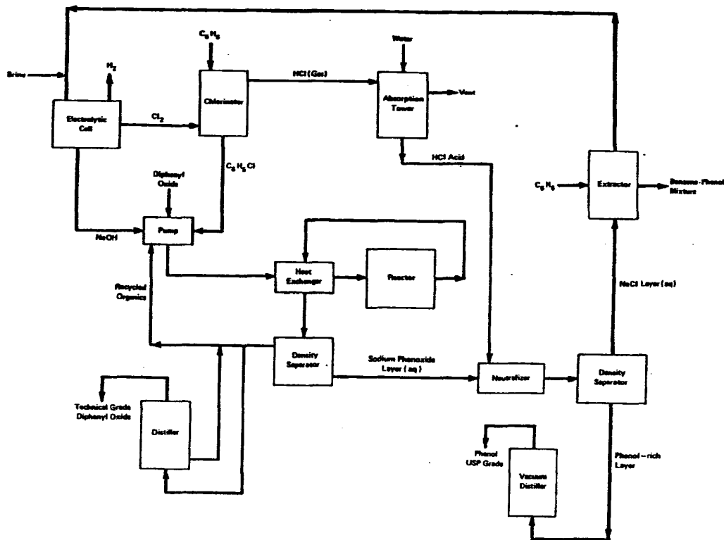
Figure IV-3. Diphenyl Oxide from Chlorobenzene - Phenol Process
