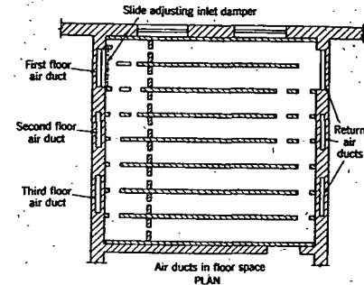
FIG. 2. AIR DUCTS FOR FLOOR HEATING
