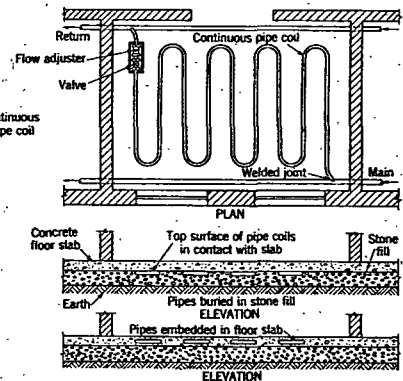
FIG. 4. COILS EMBEDDED IN FLOORS
