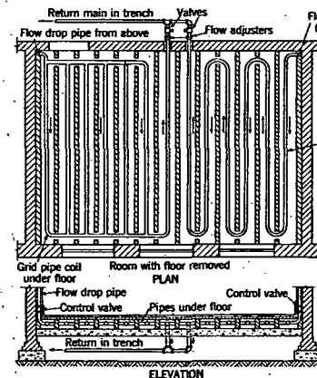
FIG. 3. CONTINUOUS COIL IN FLOOR
