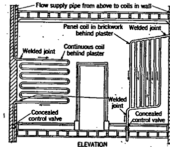
FIG. 1. COILS IN WALL SURFACES
