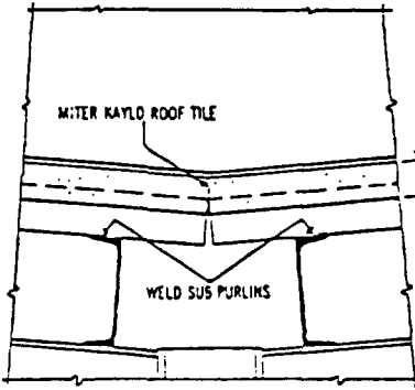
VALLEY SECTION
