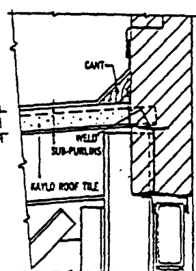
PARAPET SECTION S/S SURF PERPENDICULAR TO WALL
