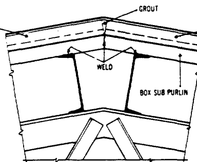
RIDGE SECTION
