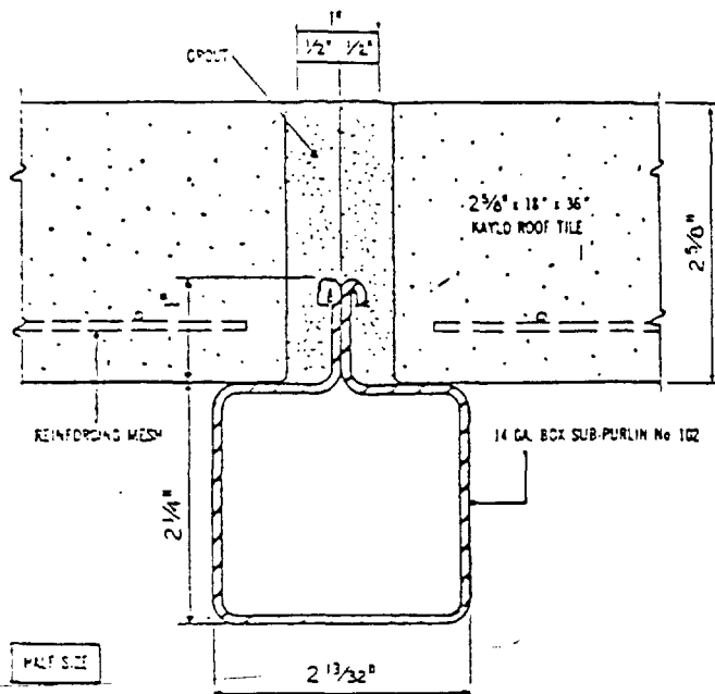
SECTION THROUGH JOINT
