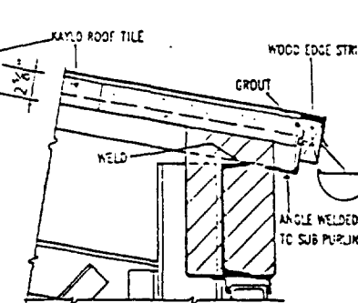
EAVE SECTION SKELETON FRAME
