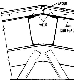
RIDGE SECTION
