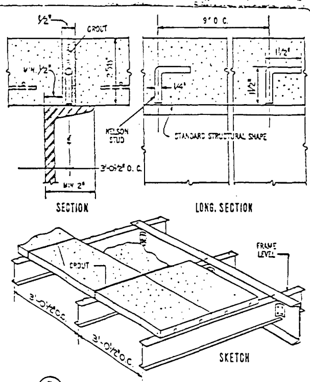
Detail B STANDARD STRUCT. SHAPES
