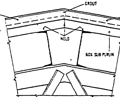
RIDGE SECTION
