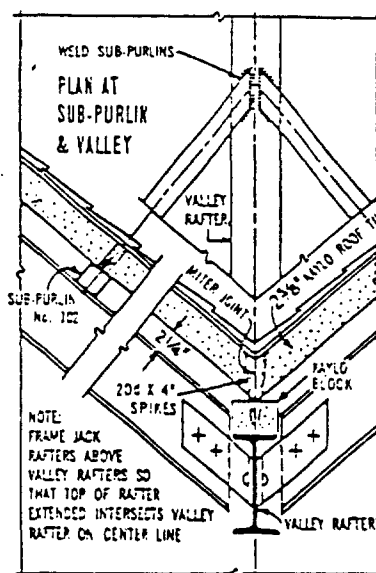
VALLEY DETAIL
