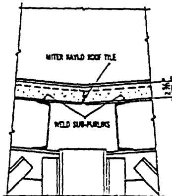
VALLEY SECTION
