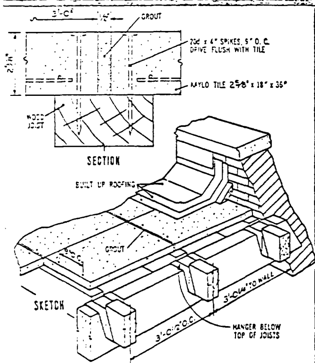
Detail C SLOW BURNING CONST.
