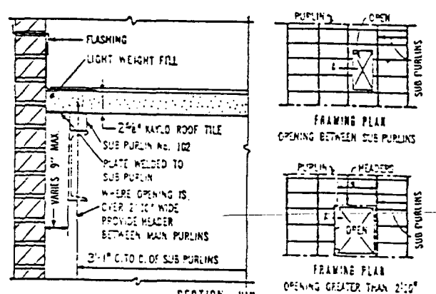
SECTION—"A" FRAMING AROUND OPENINGS (USING SUB-PURLIN No. 102)
