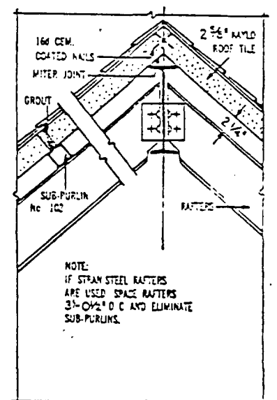
RIDGE DETAIL
