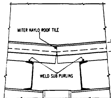
VALLEY SECTION
