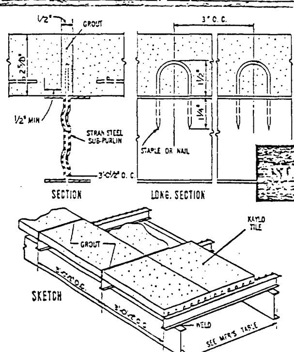
Detail D STRAN-STEEL SUB-PURLINS
