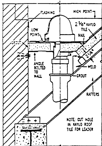
PARAPET DETAIL (SMOKING ROOF DRAIN)
