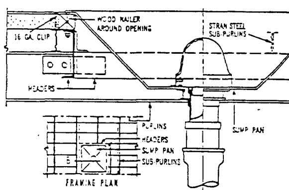
SECTION—"B" FRAMING FOR SUMP PAN (USING STRAN STEEL SUB-PURLINS)
