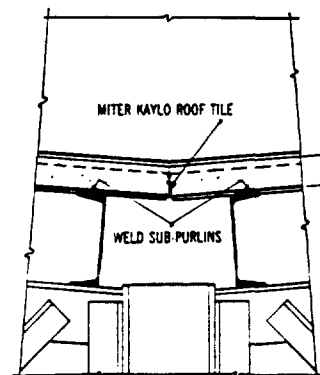
VALLEY SECTION
