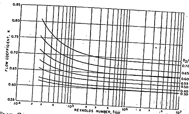
FIG. 9. FLOW COEFFICIENTS, K , FOR SQUARE-EDGED ORIFICE PLATES AND FLANGE TAPS IN SMOOTH PIPE NOTE: From Table 6 of Reference 2.
