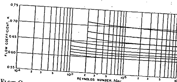
FIG. 10. FLOW COEFFICIENTS, K , FOR SQUARE-EDGED ORIFICE PLATES AND RADIUS TAPS IN SMOOTH PIPE NOTE: From Fig. 36d of Reference 3.
