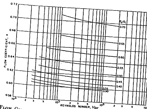
FIG. 10. FLOW COEFFICIENTS, K , FOR SQUARE-EDGED ORIFICE PLATES AND RADIUS TAPS IN SMOOTH PIPE NOTE: From Fig. 36d of Reference 3.
