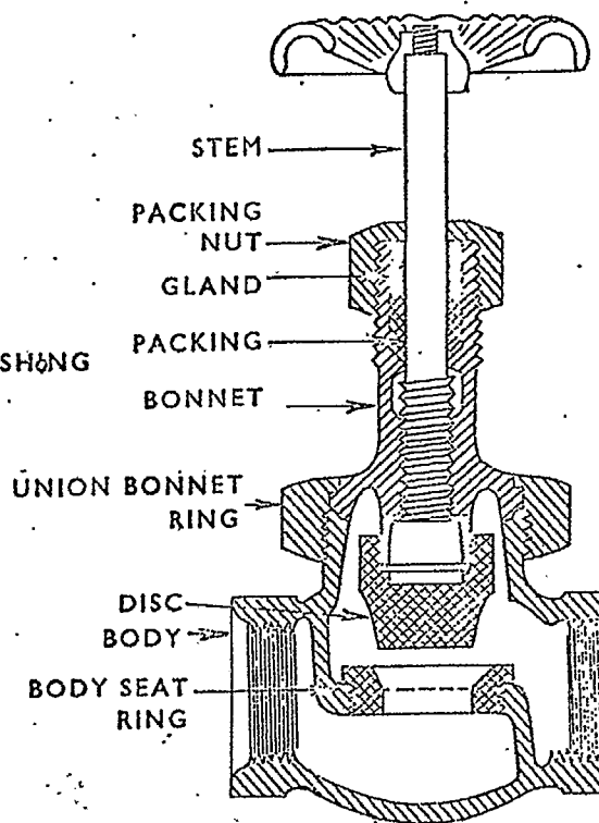
GLOBE VALVE
