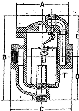
Fig. 9-1. Dimensions, No. 860T-864T.
