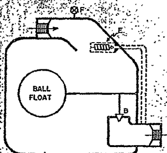
Fig. 3: Another mechanical type trap, Closed ball float design
