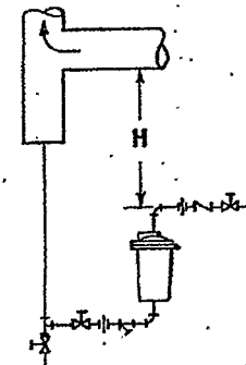
Fig. 26-1. Trap draining drip leg at riser. Distance "H" in inches ÷ 28 = psi static head for forcing water through trap.
