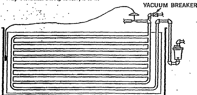
Fig. 35-3. Thermostatic controlled coil syphon drained. Use vacuum breaker check valve. Trap selection safety factor, 3 to 1 with "LV"—"CV" trap.
