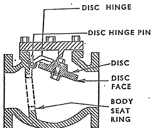
CHECK VALVE
