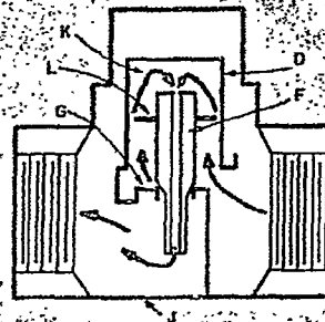
Fig. 7. This impulse design trap uses orifice-in-series principle.
