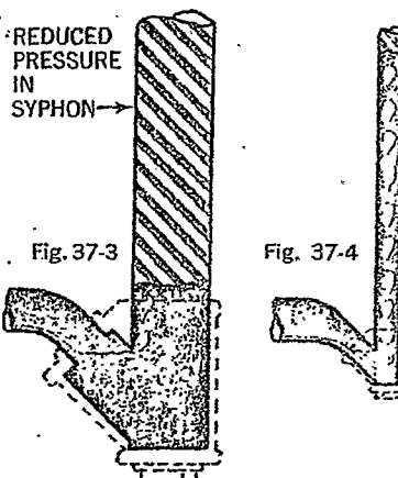
Fig. 37-3. Oversize syphon. Steam can bubble up through the condensate without changing its density. Condensate cannot reach trap until pipe is filled with condensate.
