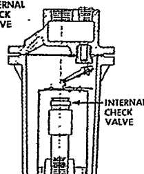
Fig. 4-6. Internal check valve installed in trap inlet.
