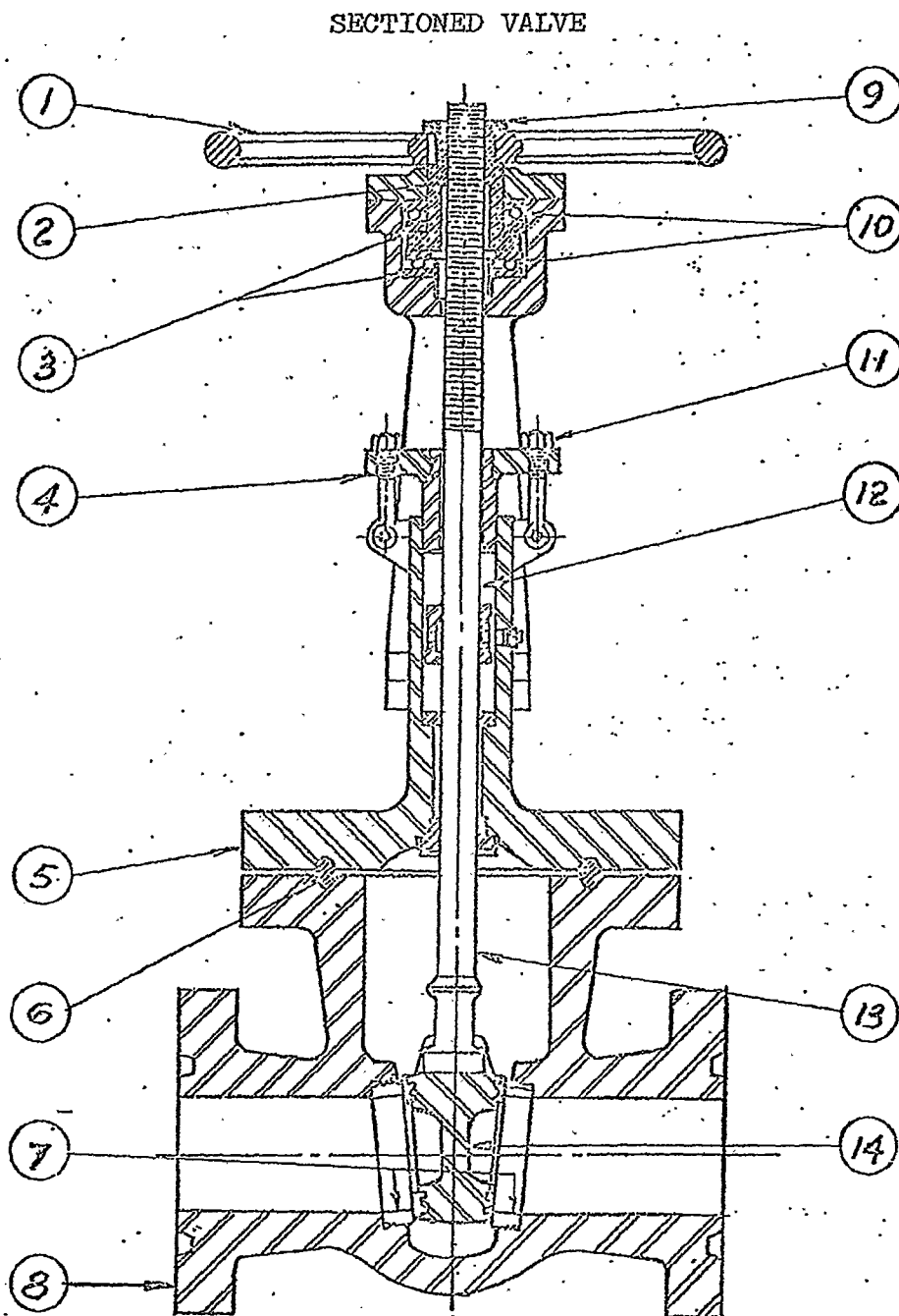
CAST STEEL GATE VALVE
