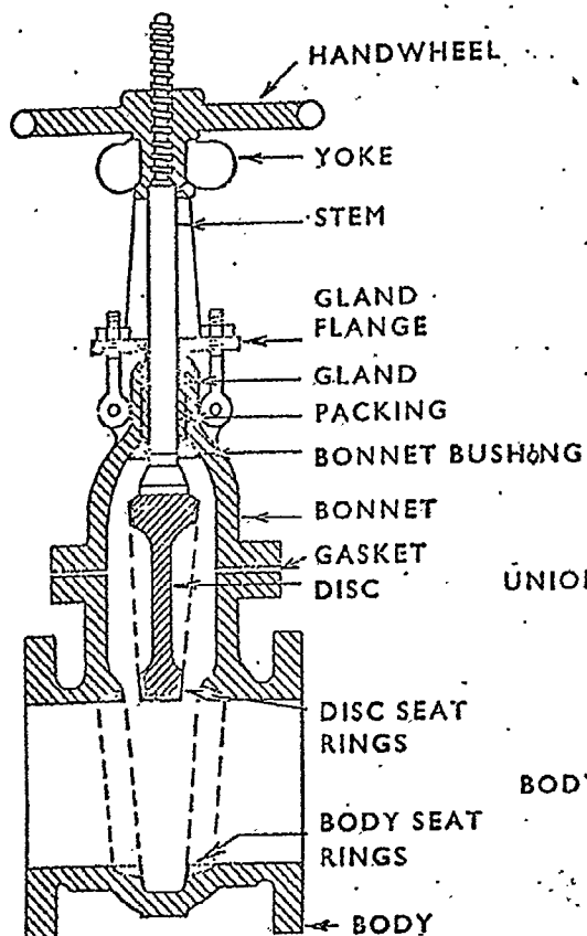
GATE VALVE
