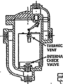
Fig. 4-6. Internal check valve installed in trap inlet.
