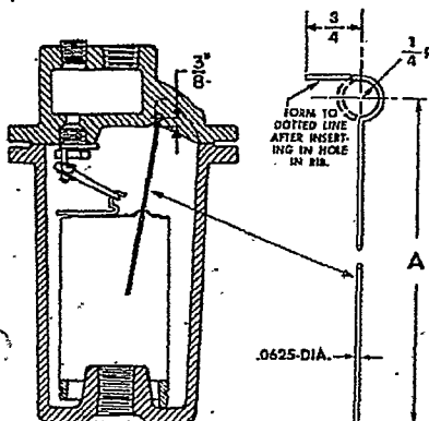
Fig. 44-1. Vent scrubbing wire for use when dirt plugs vent. Trap inlet tube must be removed.
