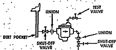
Fig. 42-1. Standard hookup No. 800-814, 880-883 traps, with shut-off valves to isolate trap during testing, inspection or repair. Unions should be at right angles—not in-line—to facilitate trap removal.
