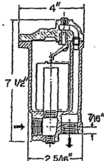
Fig. 12-2. Dimensions, No. 701 with right angle connections.
