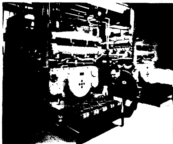
The two diesel drive generators, used to power American's computer room in the event of a power outage are automatically started by five 6-volt lead acid batteries connected in series.
