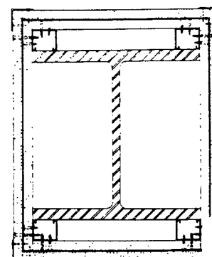
ILLUSTRATION—TWO-HOUR fire rated steel column assembly with 5/8" G-P/Bestwall Firestop.
