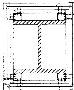
ILLUSTRATION—THREE-HOUR fire rated steel column assembly with 5/8" G-P/Bestwall Firestop.
