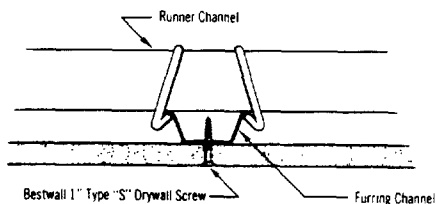
Ceiling Furring Detail
