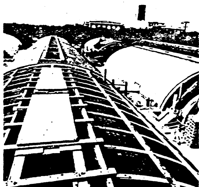
The vaulted roof shell in the right foreground has the lead sheet roofing completed. In the background, workmen are installing the calcium lead alloy on another vault.
