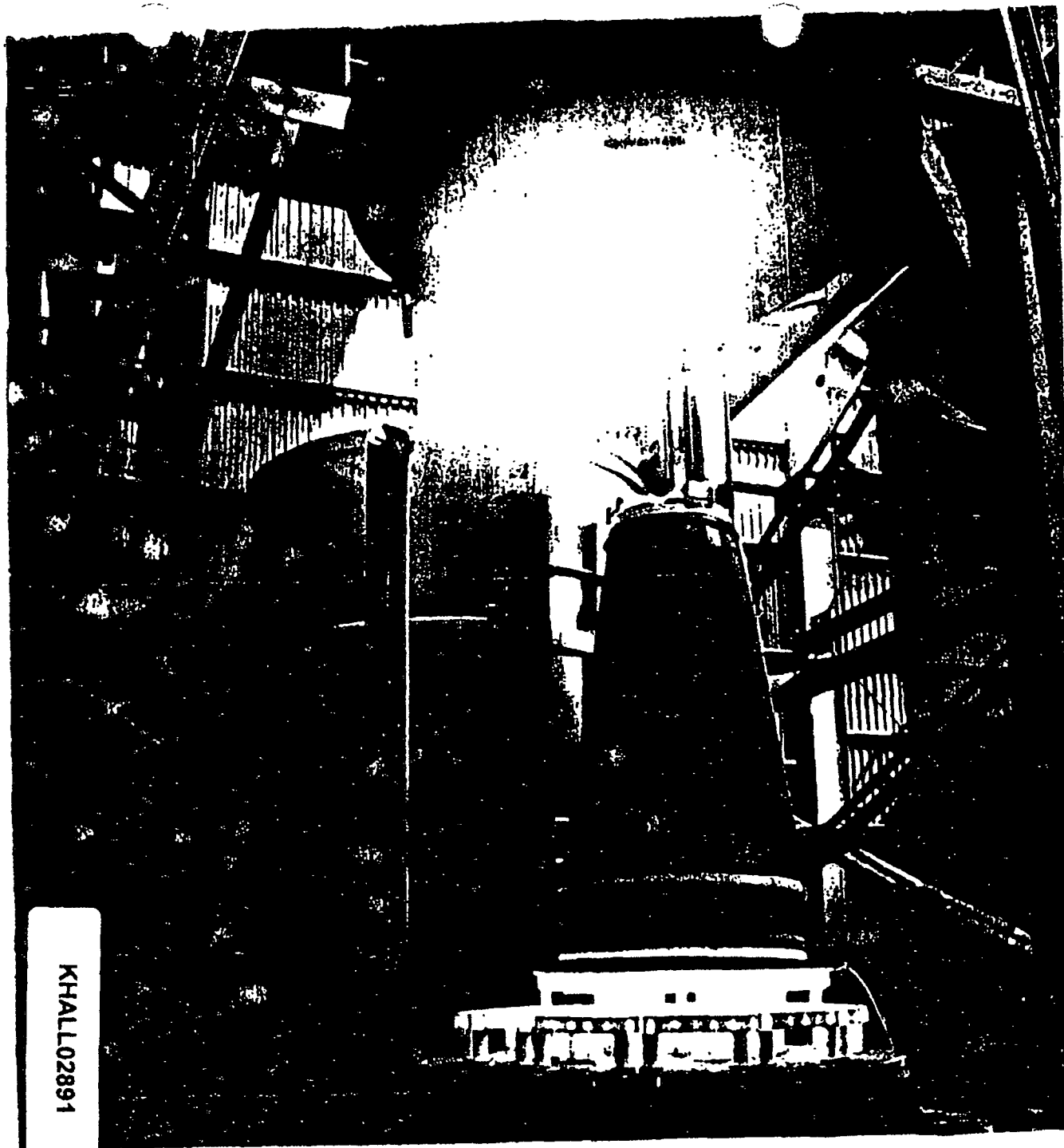
Thermalloy castings support rocket casing as heat treat furnace hood is raised.
