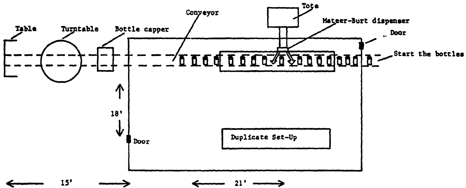
FIGURE II Pennex Pharmaceuticals Baby Powder Line
