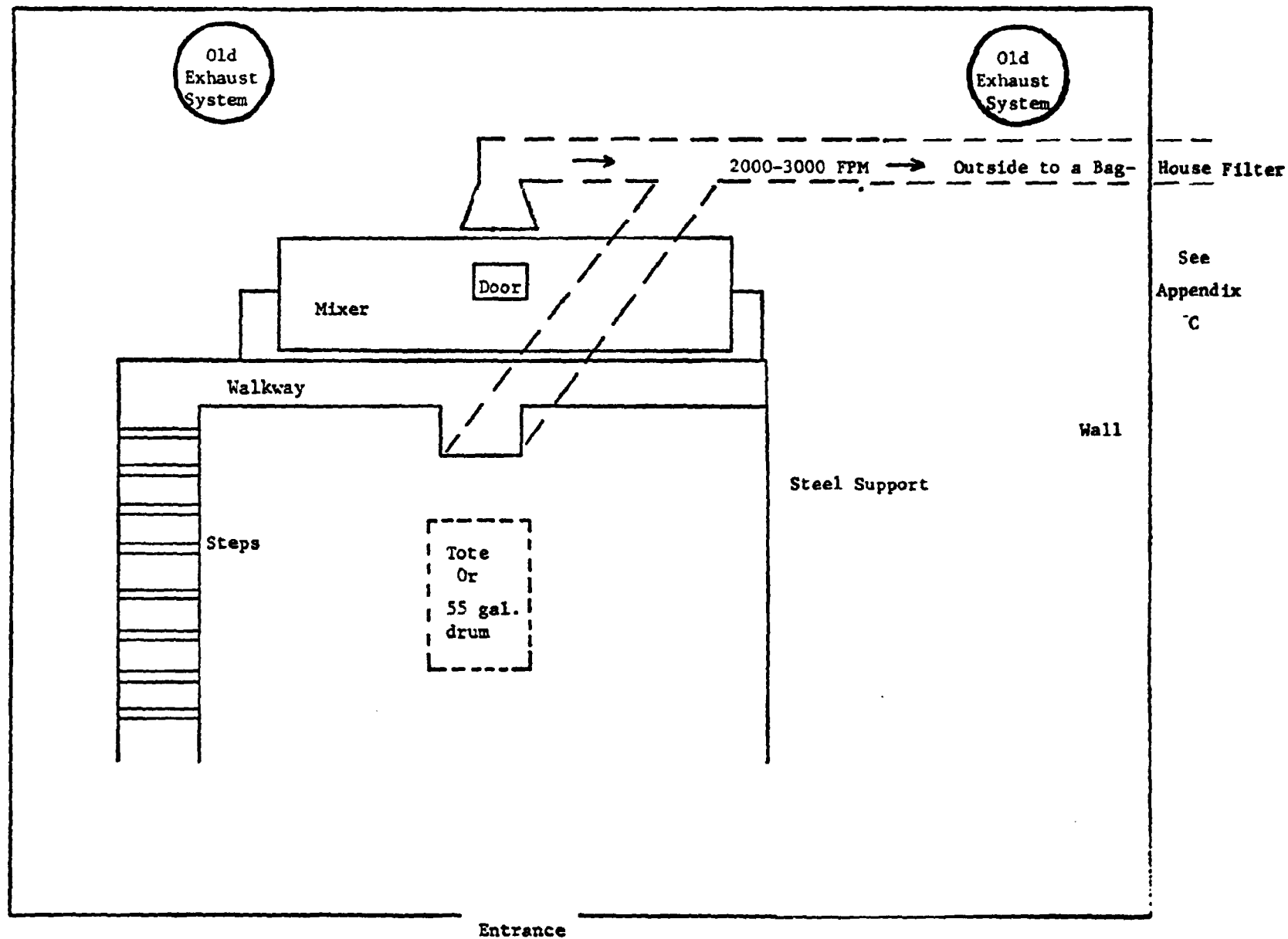
FIGURE I Pennex Pharmaceuticals Proposed Ventilation System
