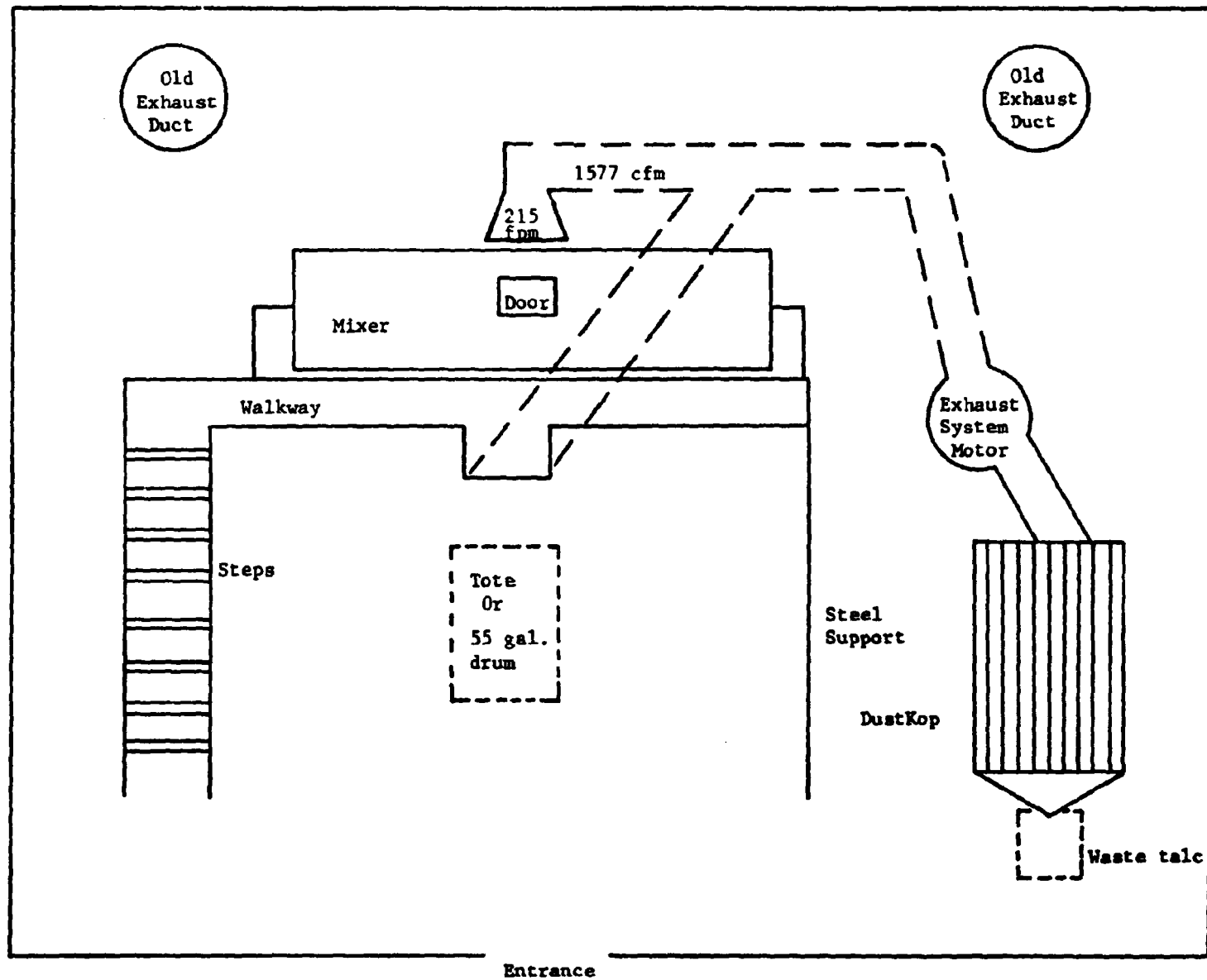
FIGURE III Pennex Pharmaceuticals Existing Ventilation System
