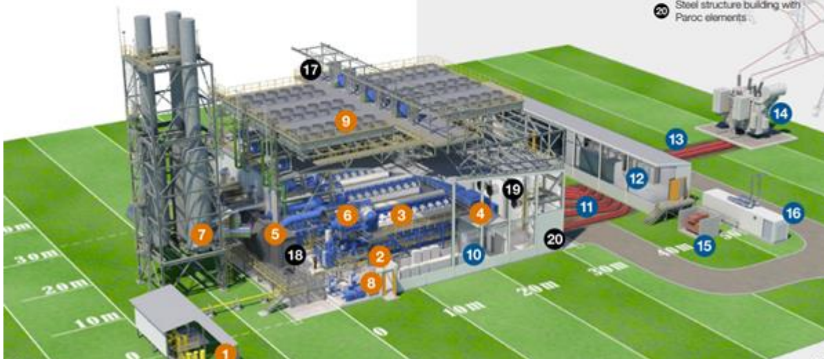
Figure 2 - schema of Combined Heat & Power system (18 p. 56)
