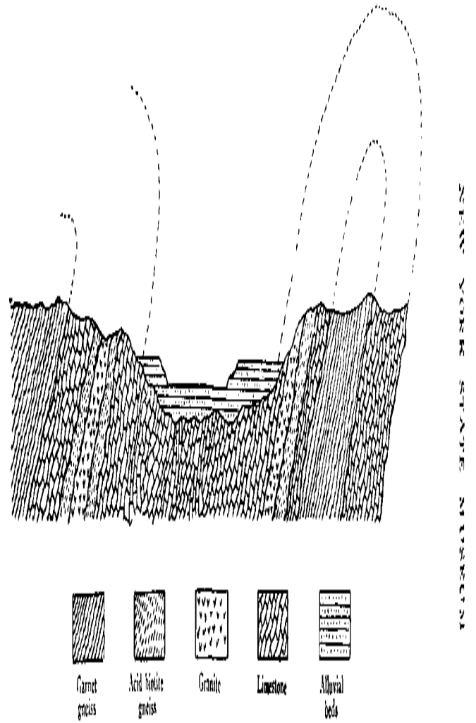
Figure 14. Section across the limestone belt at Edwards, showing folded relations of the Grenville strata. The central belt is a syncline, bordered by compressed anticlines.
