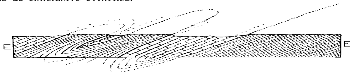
Figure 11 Section E—E, showing two infolded minor synclines of limestone, between anticlines of garnet-gneiss, on the flank of the great fold of garnet-gneiss which is partially represented at the right.
