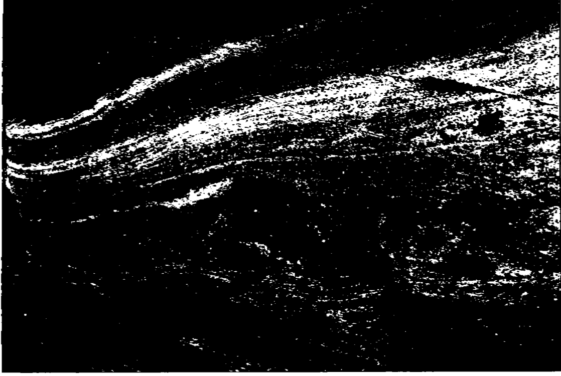
Folding and banding of impure Greville limestone, Edwards.
