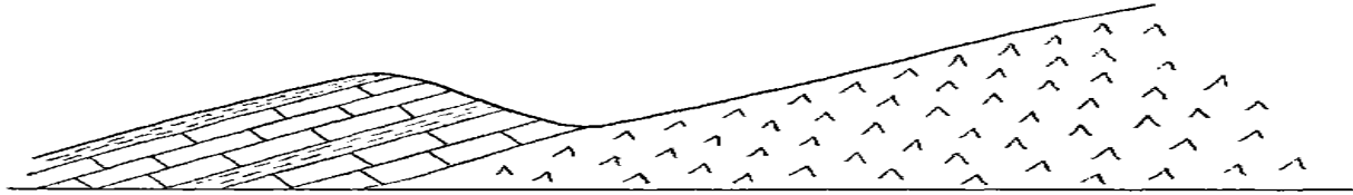
Figure 3 Section of Grenville limestone hog-back ridge at south end of Reservoir Hill granite sill.
