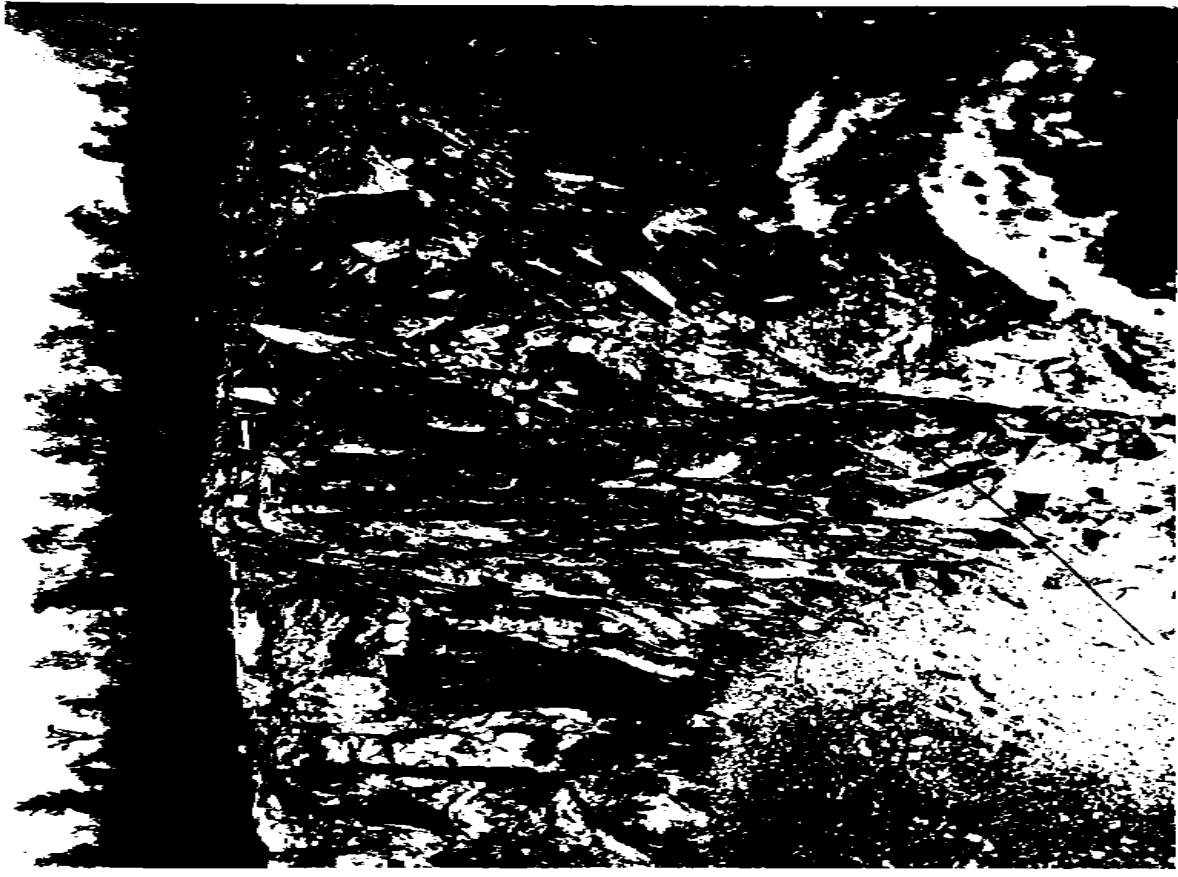
Gouverneur limestone in Corrigan & McKenney pit north of Gouverneur looking west along north wall of pit to the northwest corner. Solid, massive, white, pure limestone.
