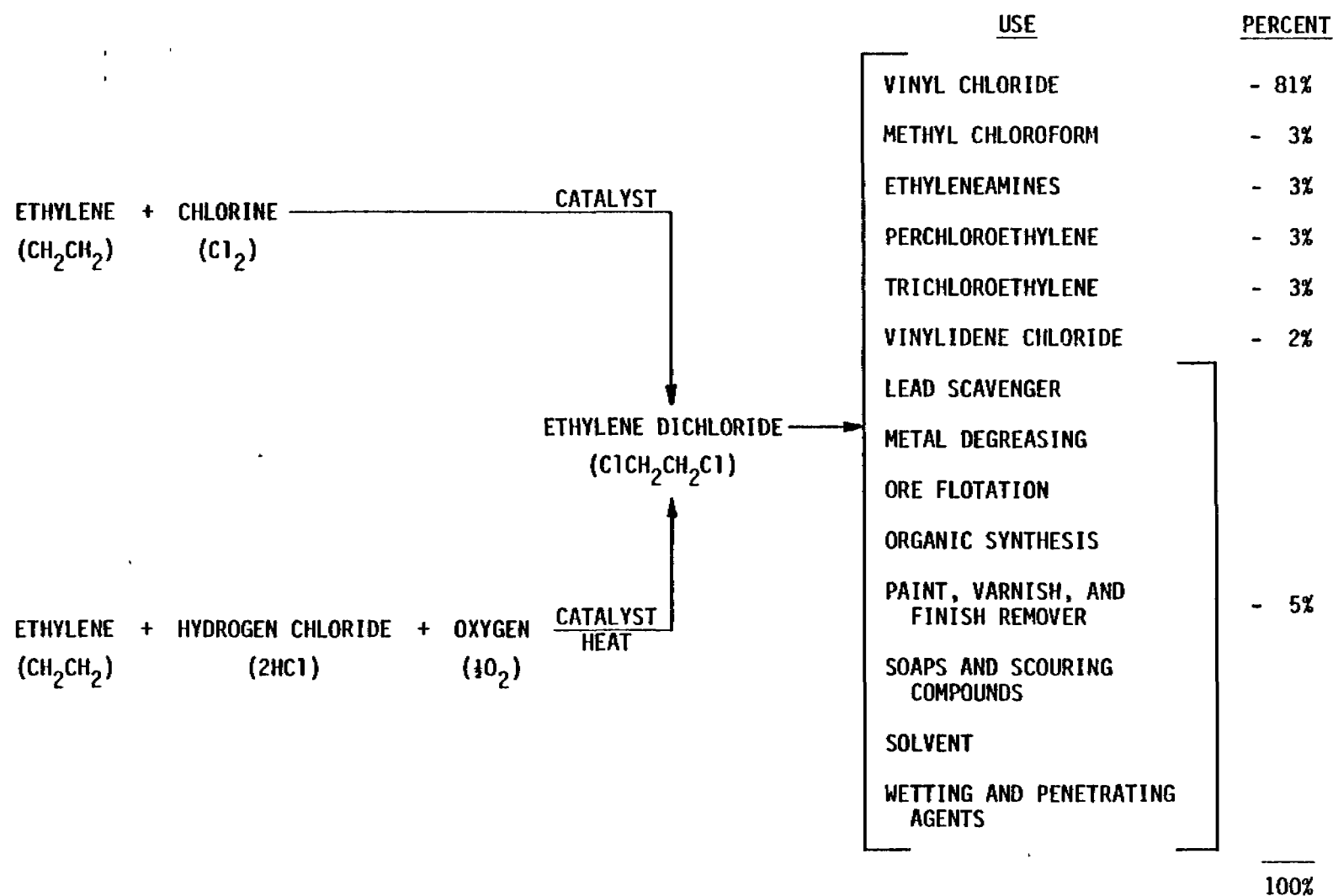
Figure 1. Chemical use tree for ethylene dichloride. 4
