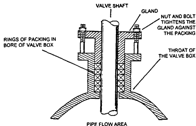
FIGURE 1. Diagram of steam pipe valve containing packing.
