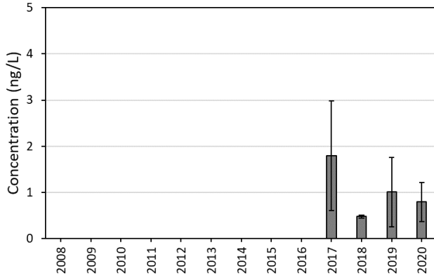
6:2 FTS (LOBPTN)
