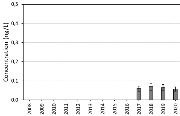
PFPeS (NOORDWK2)
