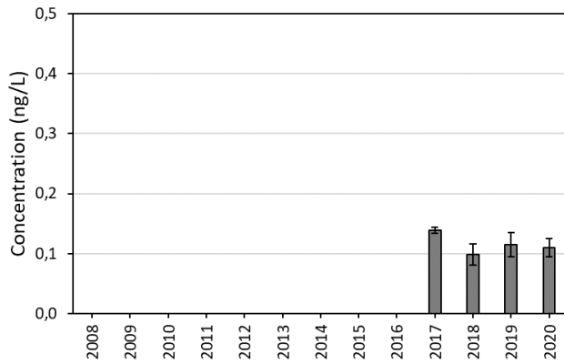
PFPeS (BOCHTVWTM)
