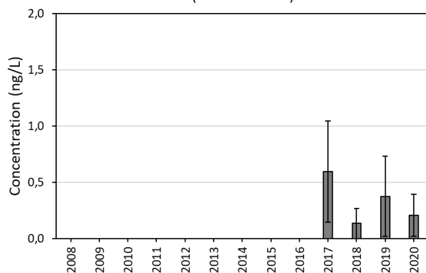
6:2 FTS (BOCHTVWTM)
