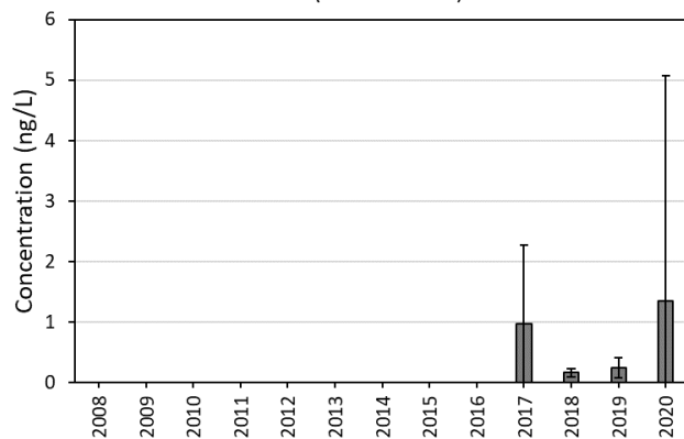
6:2 FTS (NOORDWK2)
