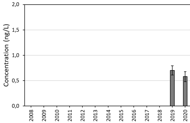
PFHpA (DREISR)
