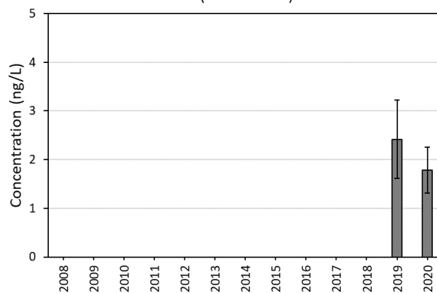
GenX (MARKMMDN)
