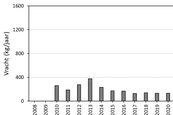
PFOA LOBPTN
