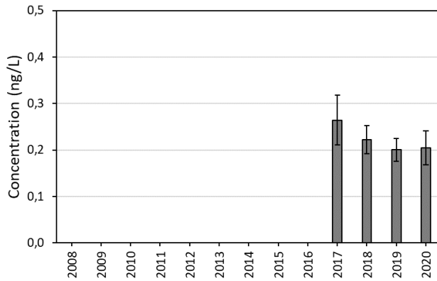
PFPeS (MAASSS)
