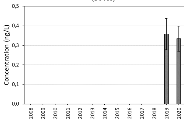
PFNA (BOVSS)
