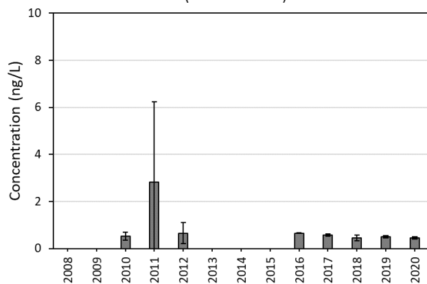
PFHxS (NOORDWK2)
