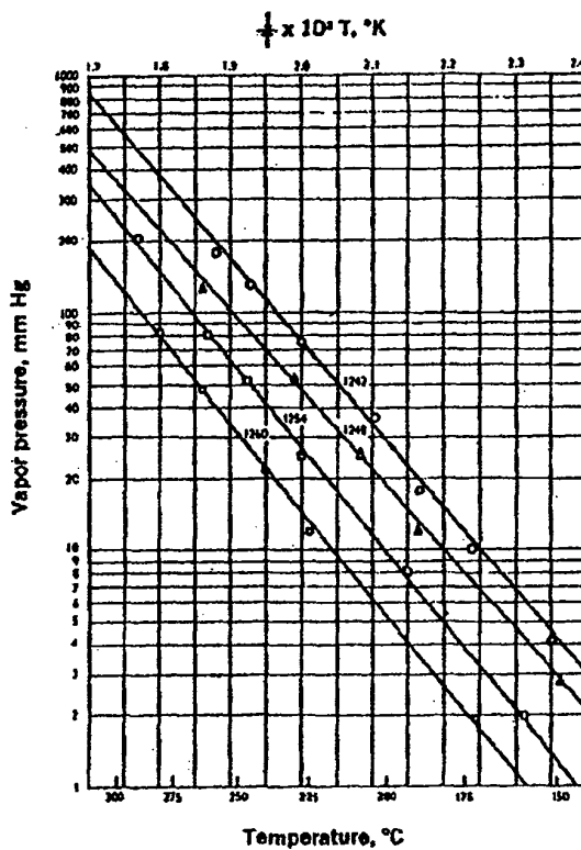
Fig. 2 — Vapor Pressures of Aroclor® Plasticizers
