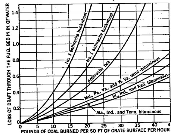
FIG. 8. DRAFT REQUIRED AT DIFFERENT RATES OF COMBUSTION FOR VARIOUS KINDS OF COAL.
