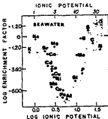
Fig. 2. Elemental enrichment factors in seawater, related to the ionic potential of the elements.
