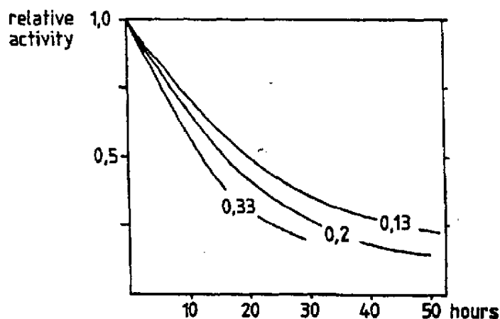
Figure 1: Relative vinyl chloride degrading activity by non-growing Mycobacterium L1 at different biomass concentrations (mg C/ml)
