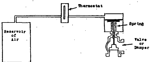
FIG. 61. EXAMPLE OF THERMOSTAT USING OUTSIDE POWER
