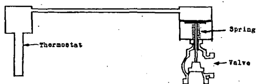
FIG. 60. EXAMPLE OF UNIT TYPE THERMOSTAT
