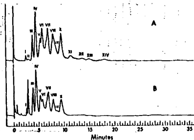
Fig. 7. Resin powder extract indicating the presence of PCB's of the Aroclor 1254 type. Chromatogram A: 5 ng. of Aroclor 1254 numbered 1 to XIV as in chromatogram B of Figure 1. Chromatogram B: The equivalent of 0.02 mg. of resin powder extract (hexane portion of Florisil split), numbered 1 to XIV as in Aroclor 1254. GLC parameters as in Figure 1
