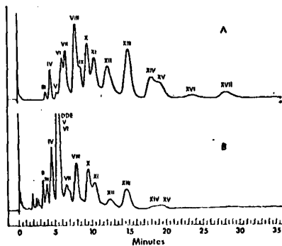
Fig. 6. Typical sample indicating the presence of PCB's of the Aroclor 1260 type in a duckling from the Toronto area. Chromatogram A: 5 ng. of Aroclor 1260 numbered 1 to XVII as in chromatogram B of Figure 3. Chromatogram B: the equivalent of 0.35 mg. of duck sample (hexane portion of Florisil split). Note the DDE contribution to PCB peak V. GLC parameters as in Figure 1
