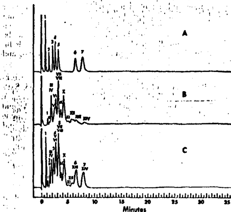
Fig. 2. Separation of PCB's and organochlorine pesticides on polar phase column (five percent DECS/two percent H_2PO_4 ). Chromatogram A: standard mixture of organochlorine pesticides with same amounts as in Figure 1; peak numbers: 1 = heptachlor and aldrin, 2 = lindane, 3 = heptachlor epoxide, 4 = DDE, 5 = dieldrin, 6 = DDT, 7 = DDD. Chromatogram B: 5 ng. of Aroclor 1254 (the 14 major peaks are numbered 1 to XIV as in chromatogram B of Figure 1, assuming that the order of elution is unchanged). Chromatogram C: combination of organochlorine standard pesticide mixture and Aroclor 1254. Other GLC parameters as in Figure 1
