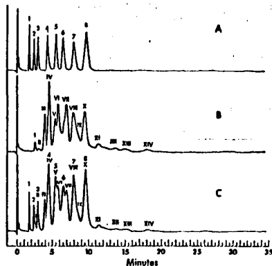
Fig. 1. PCB interference with organochlorine pesticide residue analysis on four percent SE-30/six percent QF-1 on 60/80 mesh Chromosorb W, \frac{1}{8} " x \frac{1}{8} " stainless steel column. Chromatogram A: standard mixture of organochlorine pesticides; peak numbers: 1 = 0.08 ng. of lindane, 2 = 0.10 ng. of heptachlor, 3 = 0.10 ng. of aldrin, 4 = 0.14 ng. of heptachlor epoxide, 5 = 0.20 ng. of DDE, 6 = 0.20 ng. of dieldrin, 7 = 0.30 ng. of DDD, and 8 = 0.50 ng. of DDT. Chromatogram B: 5 ng. of Aroclor 1254 (the 14 major peaks are numbered I to XIV). Chromatogram C: combination of above organochlorine standard pesticide mixture and Aroclor 1254. Injector 250°C., column 200°C., detector base 250°C., N 2 at 30-35 cc./minute
