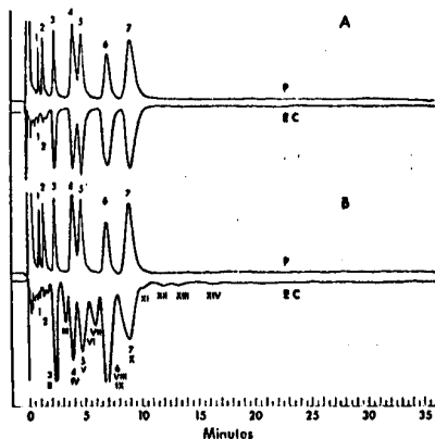
Fig. 5. Differentiation of Aroclor 1254 and organophosphorus pesticides using dual detectors and effluent split. Chromatogram A: organophosphorus standard pesticide mixture; peak numbers 1 = 1.75 ng. of phorate, 2 = 2.0 ng. of diazinon, 3 = 3.0 ng. of Ronnel, 4 = 13.0 ng. of malathion, 5 = 5.0 ng. of parathion, 6 = 15.0 ng. of methyl Trithion, and 7 = 10.0 ng. of ethion. Chromatogram B: combination of organophosphorus mixture (chromatogram A) and 10 ng. of Aroclor 1254 numbered I to XIV as in chromatogram B of Figure 1 (a compromise of the E.C. response is necessary to obtain maximum response on the phosphorus detector). P = phosphorus detector and EC = electron capture detector. Column four percent OV-100/six percent OV-210 on 60/80 mesh Chromosorb W (AW); other GLC parameters as in Figure 1
