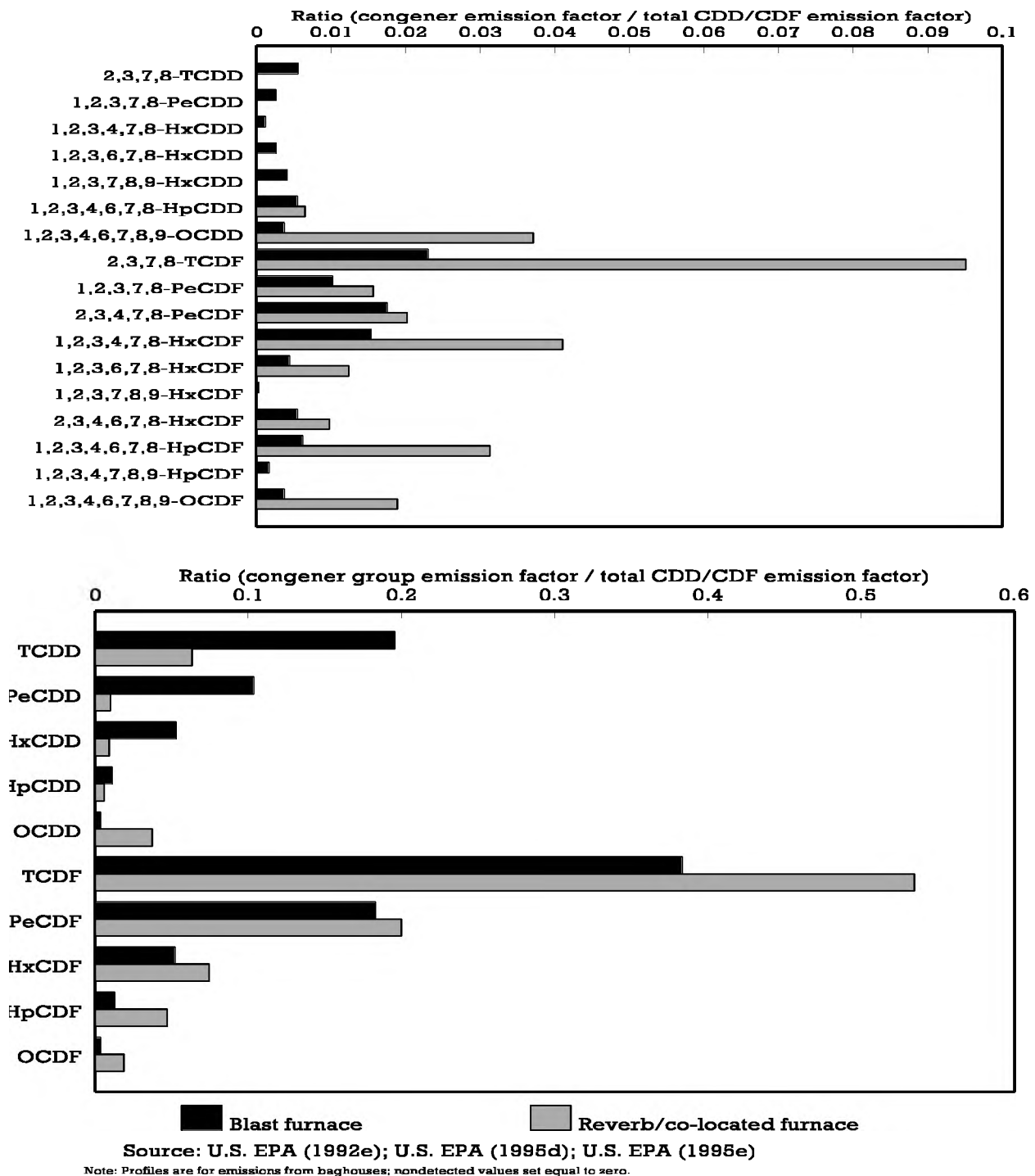
Figure 7-3. Congener and Congener Group Profiles for Air Emissions from Secondary Lead Smelters
