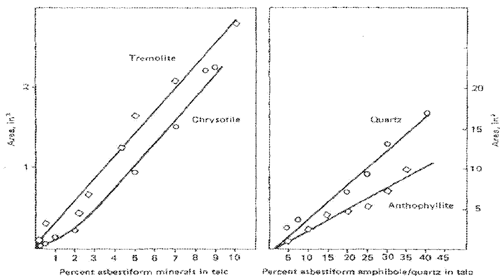
FIGURE 2. Calibration of asbestiform amphiboles and quartz in talc.
