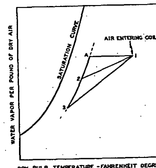
FIG. 1. PERFORMANCE OF DEHUMIDIFYING COIL
