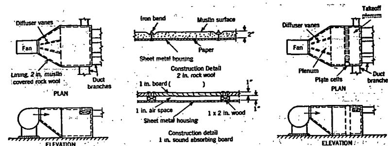
FIG. 7. ABSORPTION PLENUMS WITH AND WITHOUT SOUND CELLS
