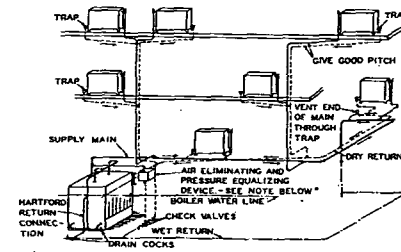
Fig. 11....Typical Up-Feed Two-Pipe System with Automatic Return Trap*
