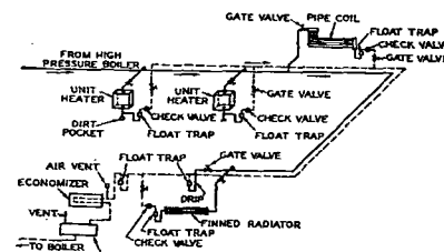
Fig. 9....Typical High-Pressure Heating System
