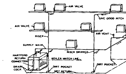
Fig. 8....Preferred Up-Feed Gravity One-Pipe Air-Vent System
